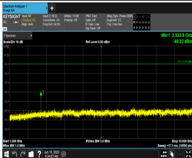
Band26-5MHz-QPSK-27015-1RB#0-Range3:1000~10000MHz
