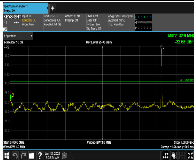
Band26-5MHz-16QAM-26815-1RB#0-Range2:30~1000MHz
