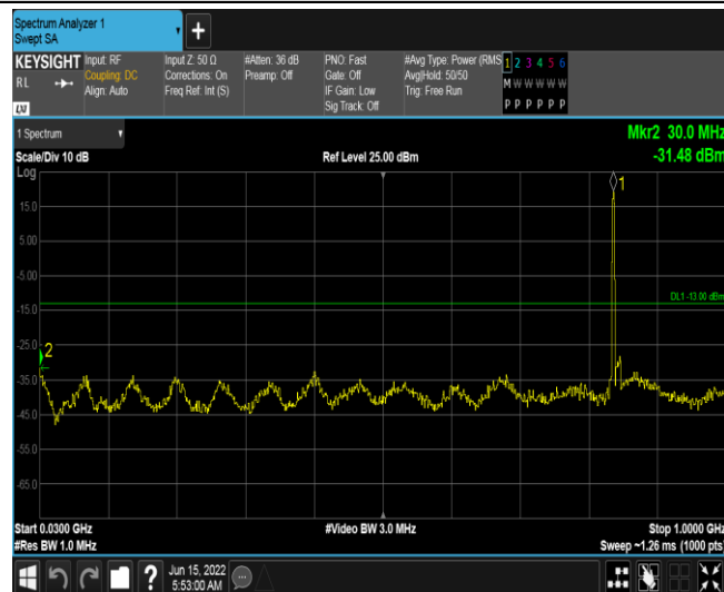
Band26-10MHz-16QAM-26990-1RB#0-Range2:30~1000MHz
