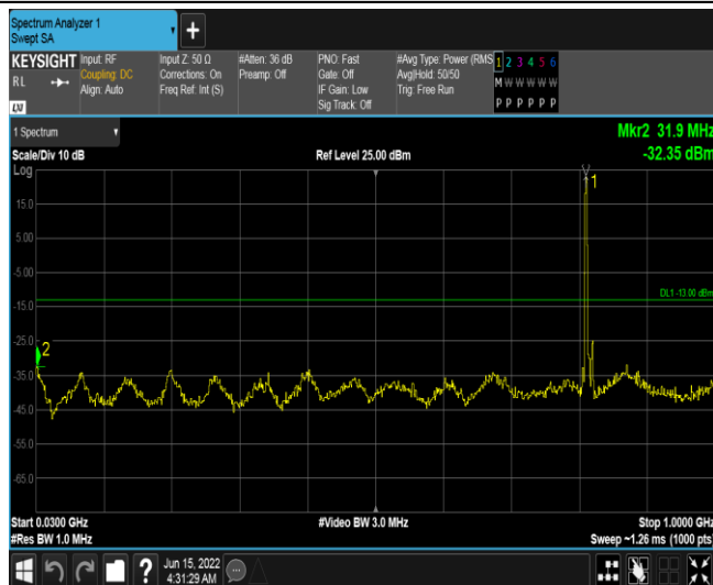
Band26-10MHz-QPSK-26740-1RB#0-Range2:30~1000MHz
