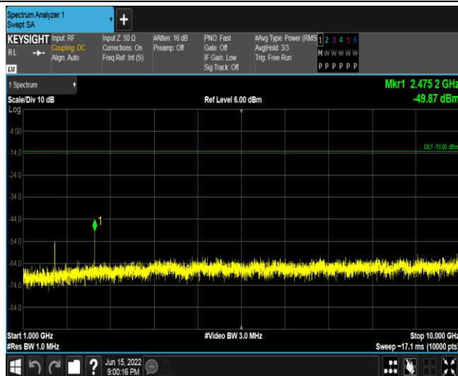
Band26-15MHz-16QAM-26865-1RB#0-Range3:1000~10000MHz
