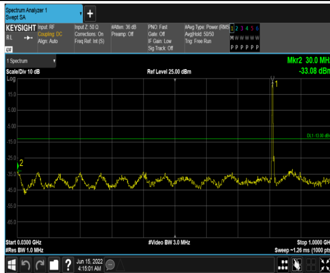
Band26-5MHz-QPSK-26715-1RB#0-Range1:30~1000MHz
