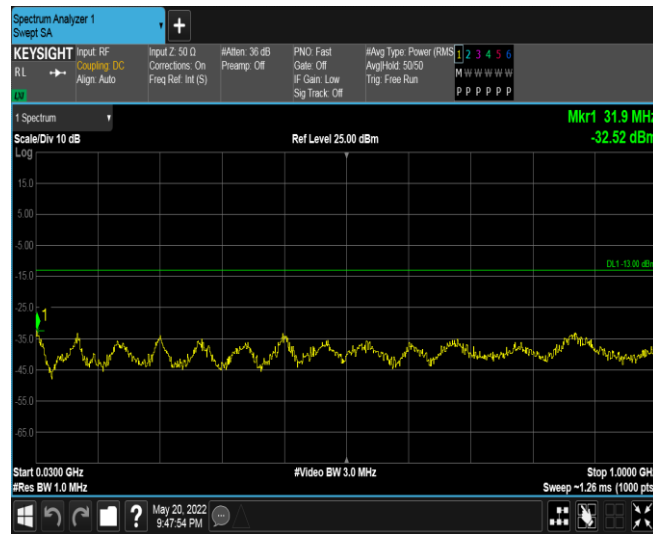
Band66-5MHz-16QAM-131997-1RB#0-Range1:30~1000MHz
