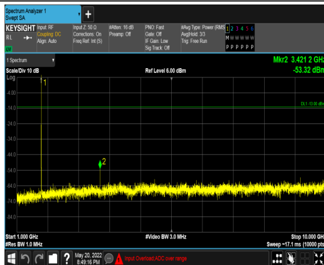
Band66-1.4MHz-QPSK-131979-1RB#0-Range3:1000~10000MHz
