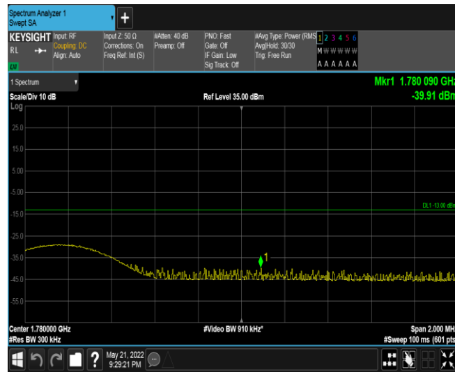
Band66-15MHz-16QAM-132597-1RB#74
