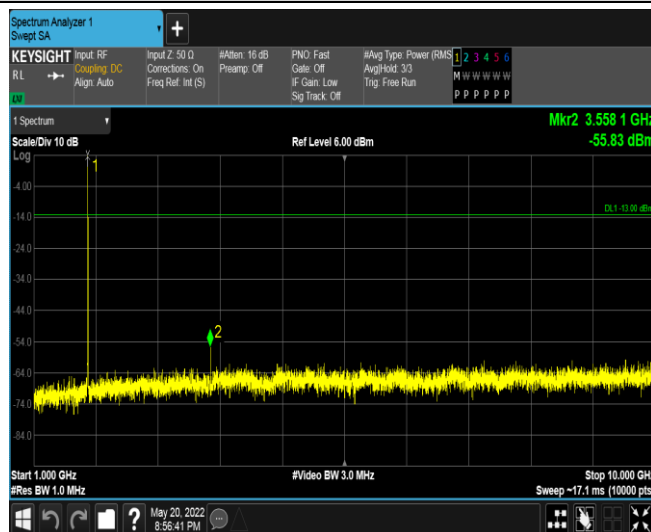
Band66-1.4MHz-16QAM-132665-1RB#0-Range3:1000~10000MHz
