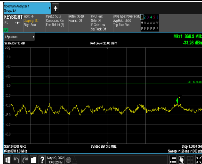
Band66-5MHz-QPSK-131997-1RB#0-Range2:30~1000MHz
