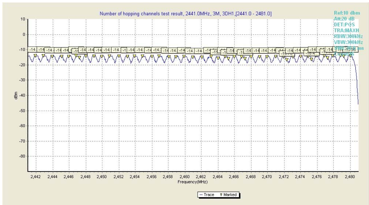
Fig33. Number of hopping channels in 2441MHz, 3Mbps,2441~2480MHz
