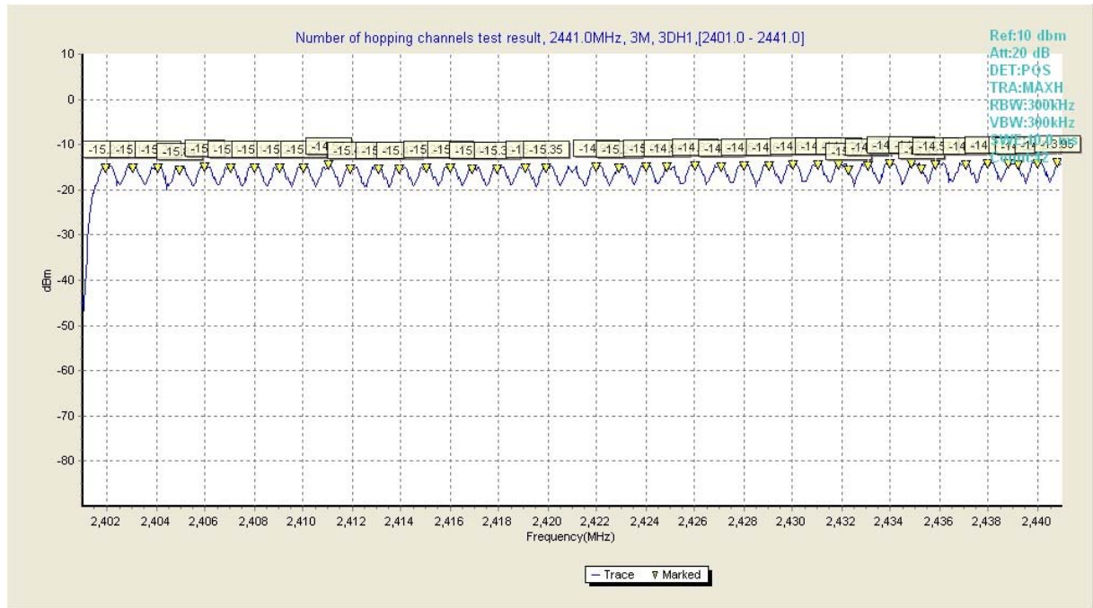
Fig32. Number of hopping channels in 2441MHz, 3Mbps,2401~2441MHz
