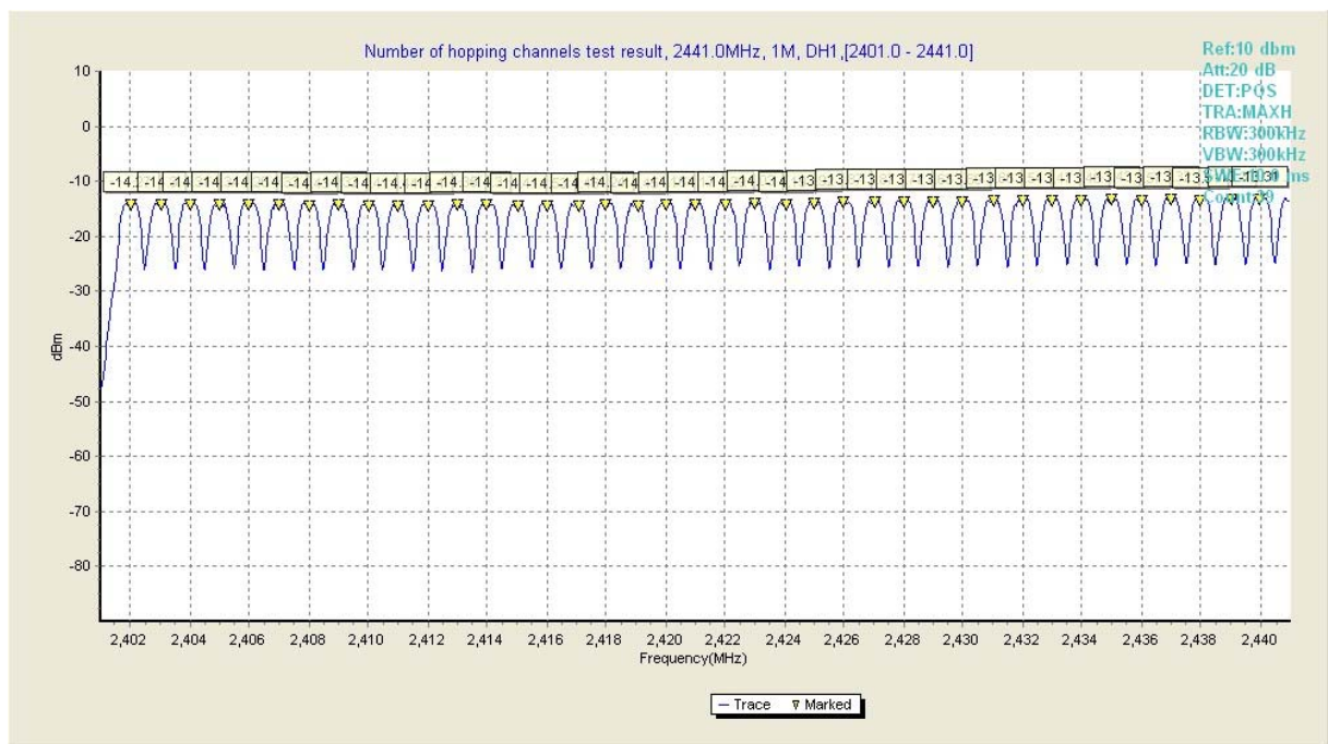
Fig28. Number of hopping channels in 2441MHz, 1Mbps,2401~2441MHz
