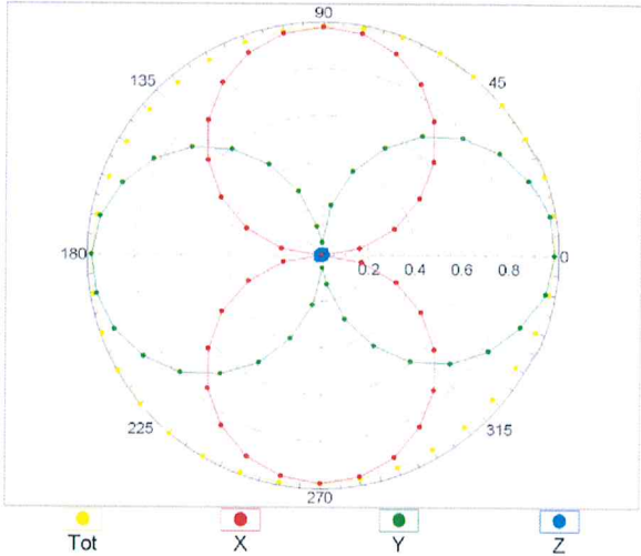
f=1800 MHz,R22,0°
