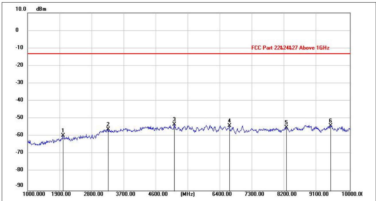
(EDGE 850MHz_ 1GHz to 10GHz _ 128 Channel _ Horizontal)
