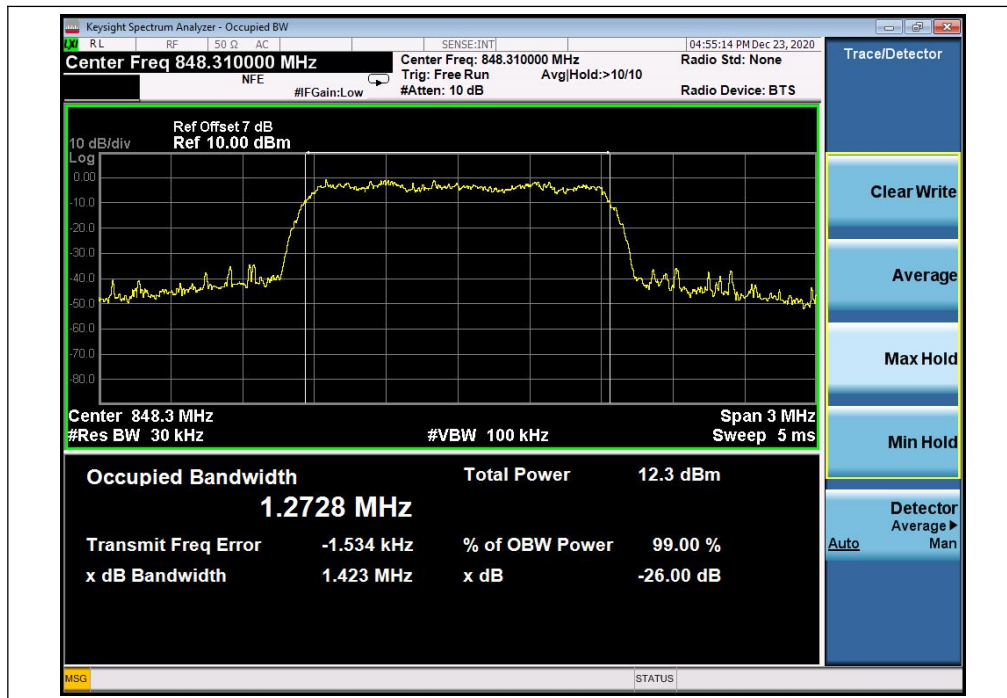
(Plot B3, 1XEVD0 Rev 0 BC0, Channel = 777)
