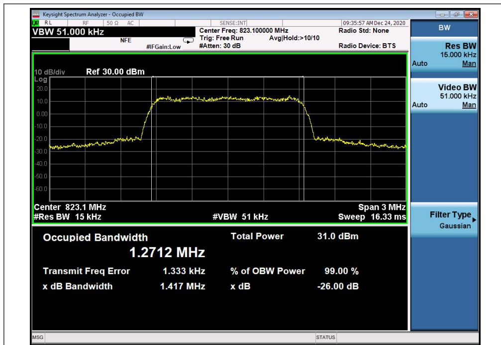
(Plot I3, 1XEVD0 Rev A BC10, Channel = 684)
