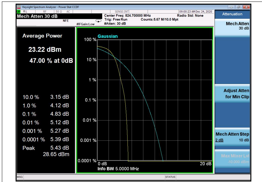
(Plot A4, EVDO Rev 0 BC0, Channel = 1013)
