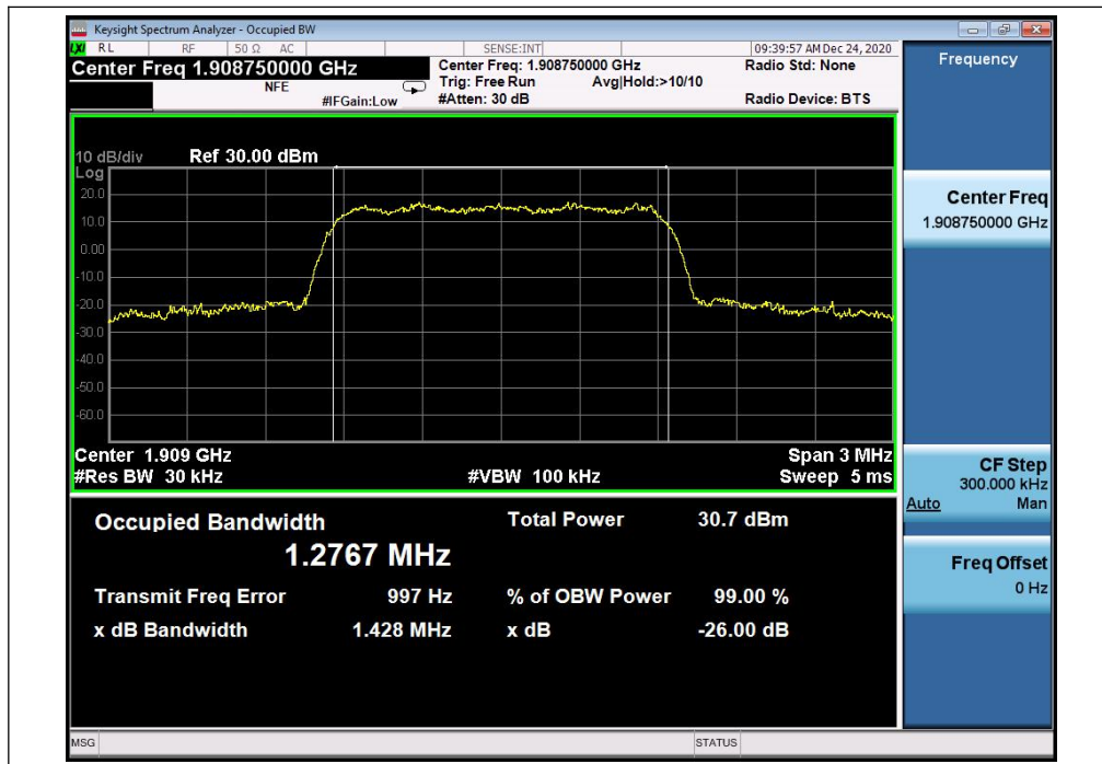
(Plot F3, 1XEVD0 Rev A BC1, Channel = 1175)
