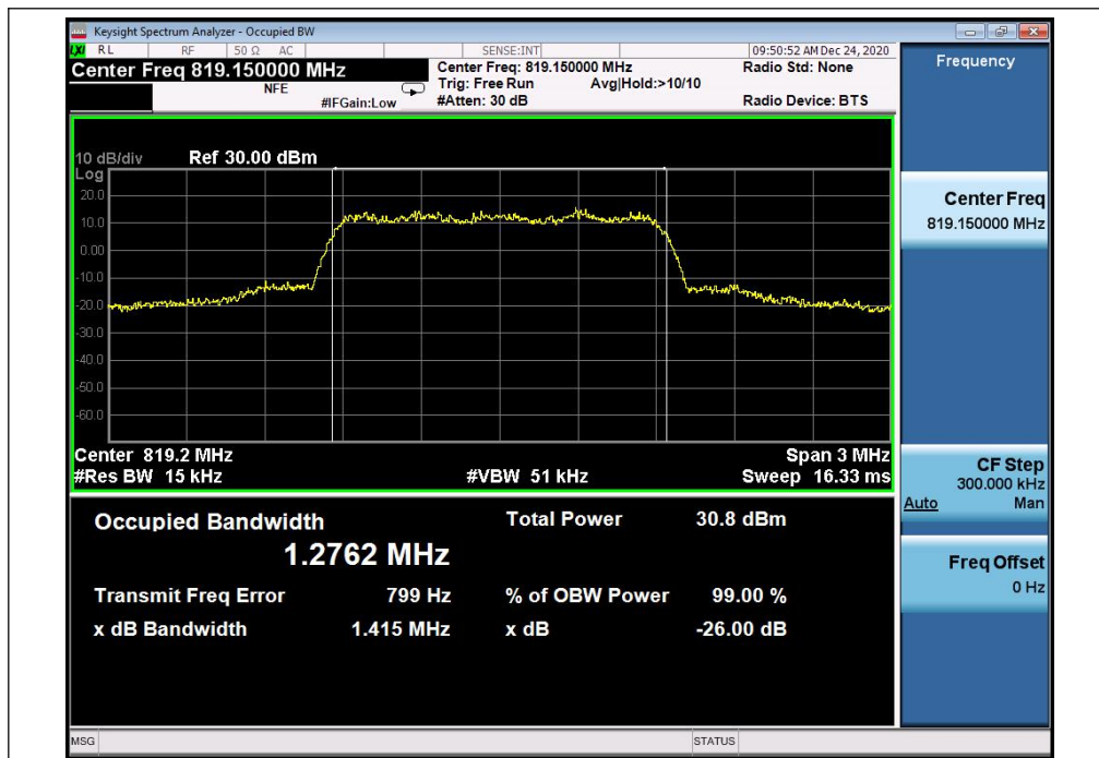
( (Plot H2, 1XEVD0 Rev 0 BC10, Channel = 526)
