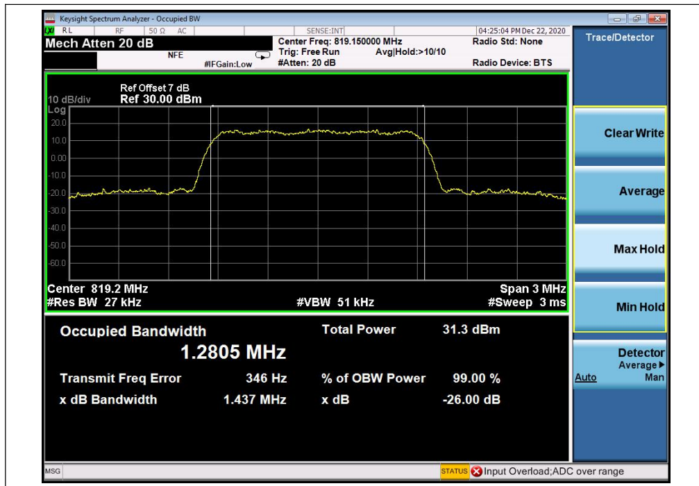
(Plot G1, CDMA BC10, Channel = 526)
