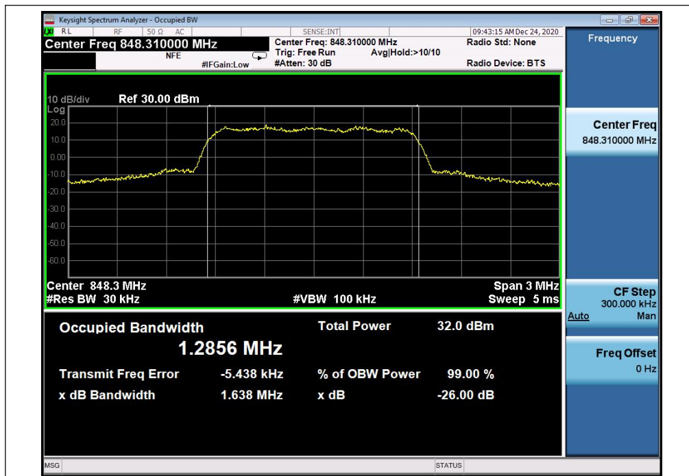
(Plot C3, 1XEVD0 Rev A BC0, Channel = 777)
