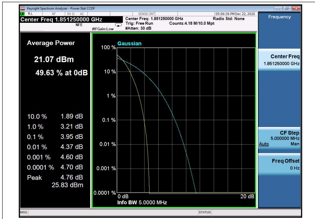
(Plot B1, CDMA BC1, Channel = 25)
