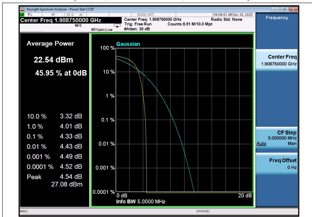
(Plot B6, EVDO Rev 0 BC1, Channel = 1175)
