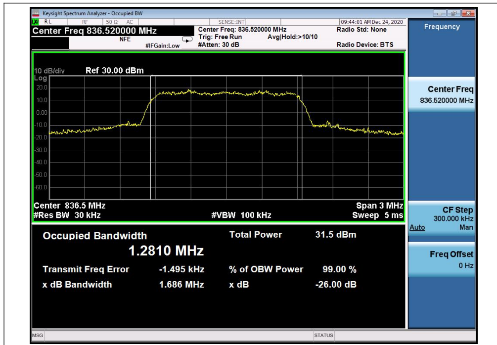
(Plot C2, 1XEVD0 Rev A BC0, Channel = 384)
