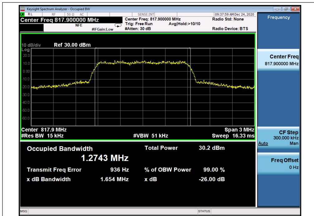
(Plot I1, 1XEVD0 Rev A BC10, Channel = 476)
