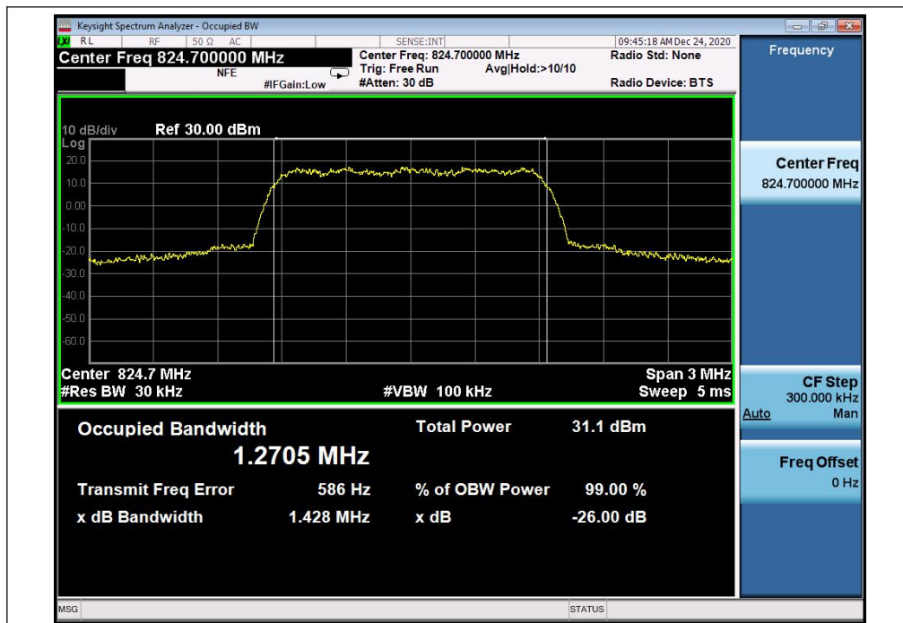
(Plot C1, 1XEVD0 Rev A BC0, Channel = 1013)
