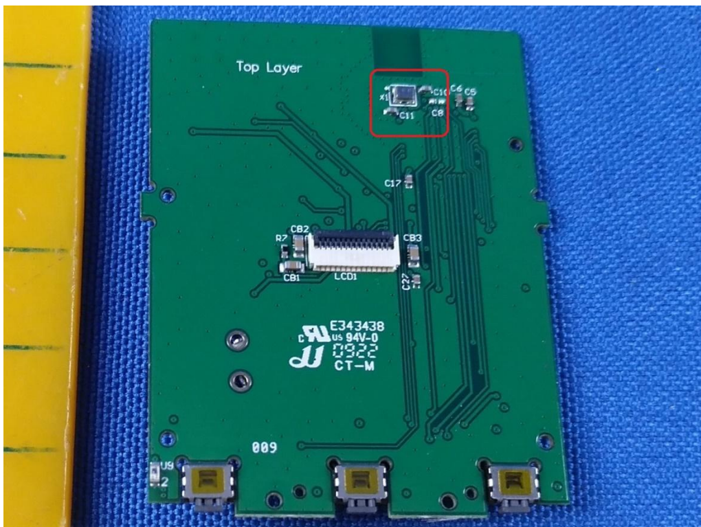
Oscillator
