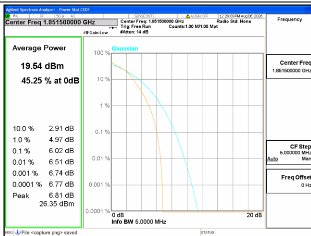
B25 / 3MHz / Low CH / 16QAM
