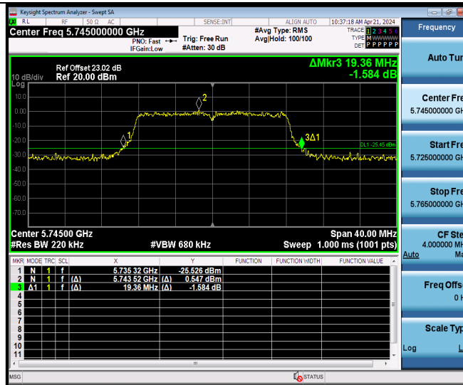
11A-CDD Ant9 5745
