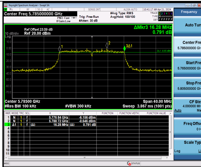
11A-CDD Ant9 5785
