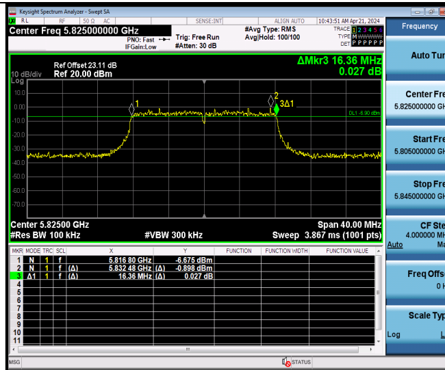
11A-CDD Ant9 5825
