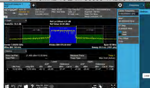
Band48-15MHz-16QAM-56665-75RB#0-PASS
