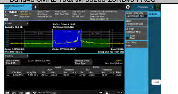
Band48-5MHz-16QAM-55990-1RB#24-PASS
