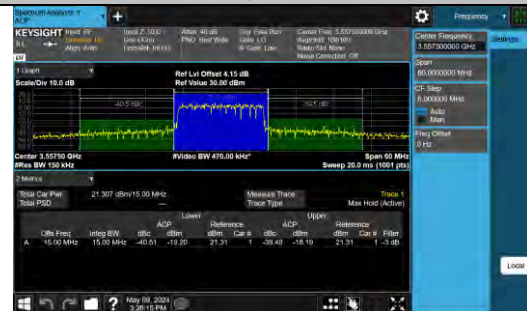
Band48-15MHz-16QAM-55315-75RB#0-PASS
