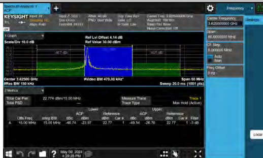
Band48-15MHz-16QAM-55990-1RB#0-PASS
