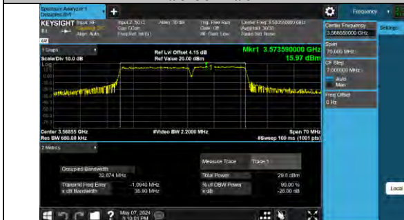
48-48-20MHz-15MHz-QPSK-QPSK-55340-55511-100RB #0-75RB#0-PASS
