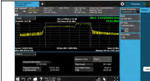
48-48-20MHz-10MHz-16QAM-16QAM-55941-56064-100 RB#0-50RB#0-PASS
