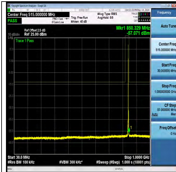
NTNV-N5-PC3-15-5-H-DFT-QPSK-Edge_1RB_Lef t-Ant2-PASS
