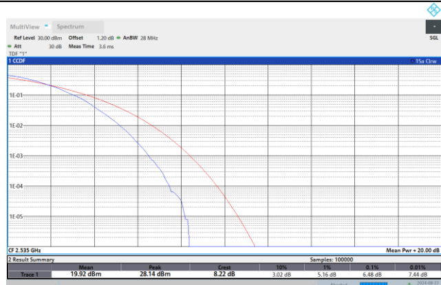
Band7-20MHz-64QAM-21100-100RB#0
