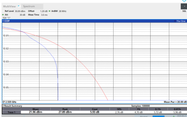
Band7-10MHz-16QAM-21100-1RB#0
