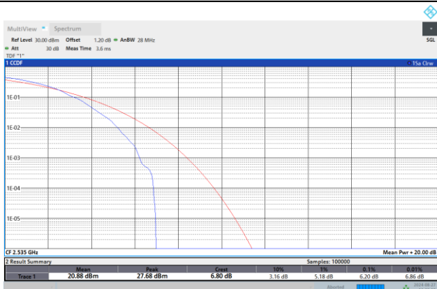
Band7-20MHz-64QAM-21100-1RB#0
