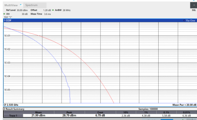
Band7-20MHz-QPSK-21350-100RB#0
