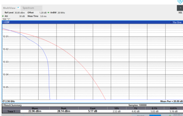
Band7-15MHz-QPSK-21375-1RB#0
