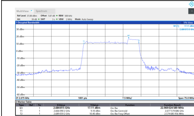
41-41-20MHz-5MHz-16QAM-16QAM-40595-40712-10ORB#0-25RB#0
