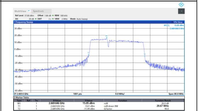
41-41-10MHz-20MHz-16QAM-16QAM-40526-40670-5 ORB#0-75RB#0
