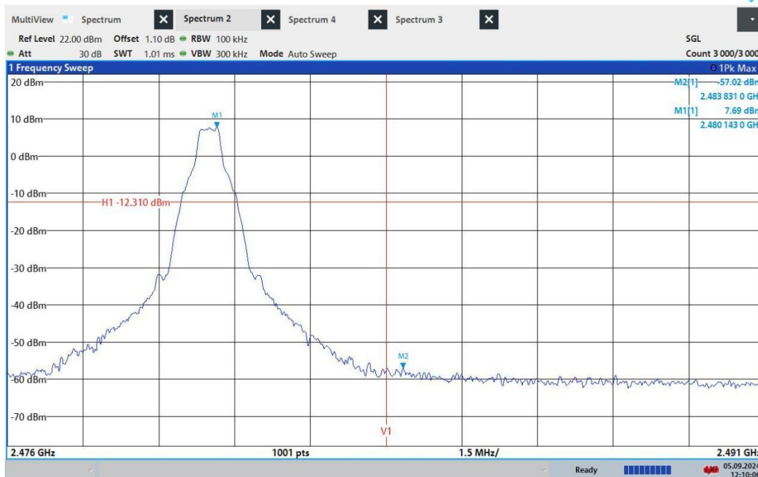
DH5_ANT0_High_2480
