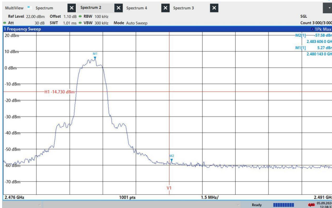
3DH5_ANT0_High_2480
