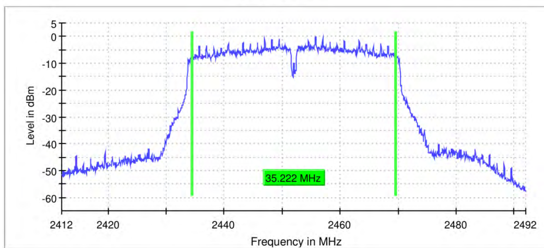
6 dB Bandwidth
