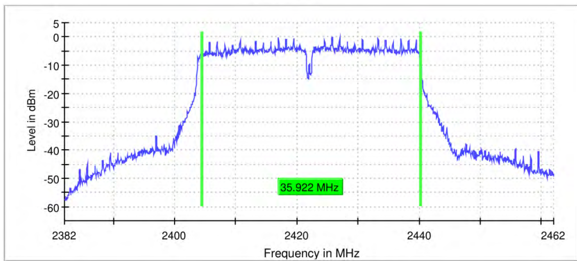
6 dB Bandwidth
