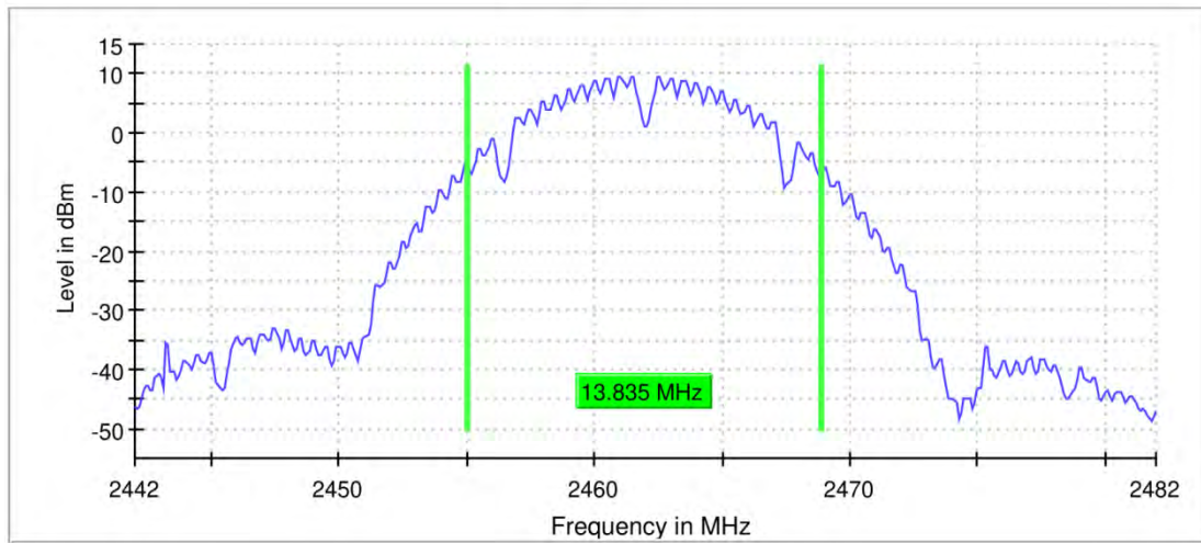
99 % Bandwidth
