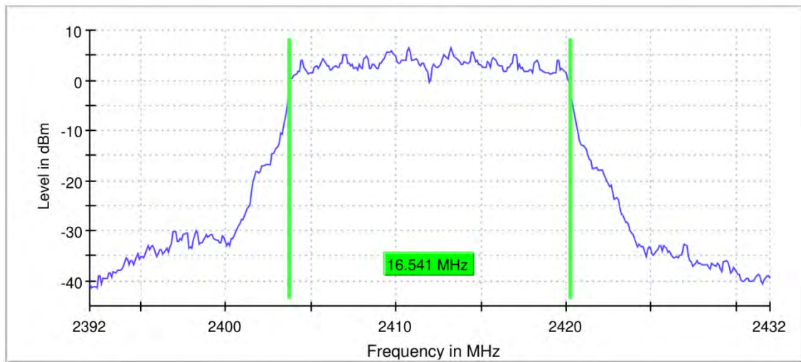
99 % Bandwidth
