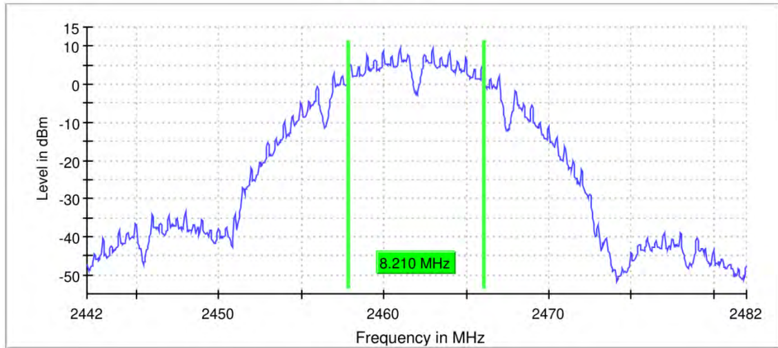
6 dB Bandwidth
