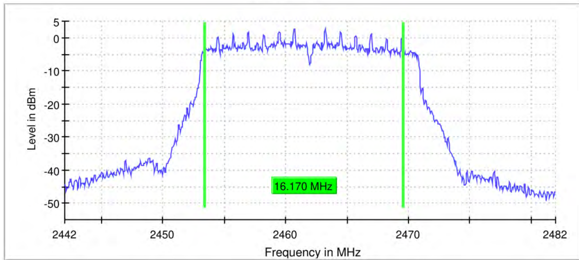
6 dB Bandwidth
