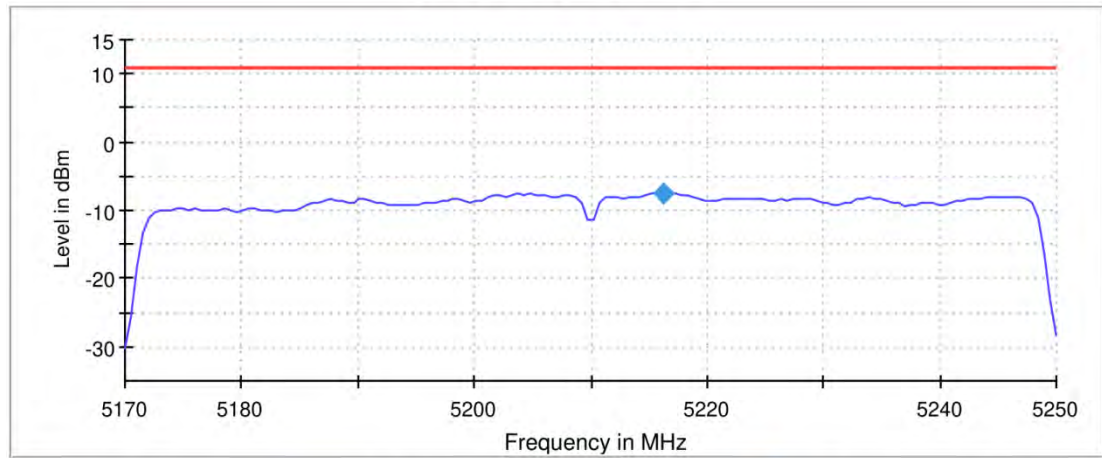
Power Spectral Density (SA-1)
