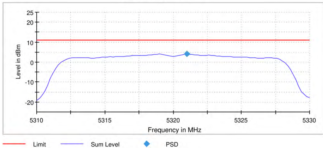
Power Spectral Density (SA-1)
