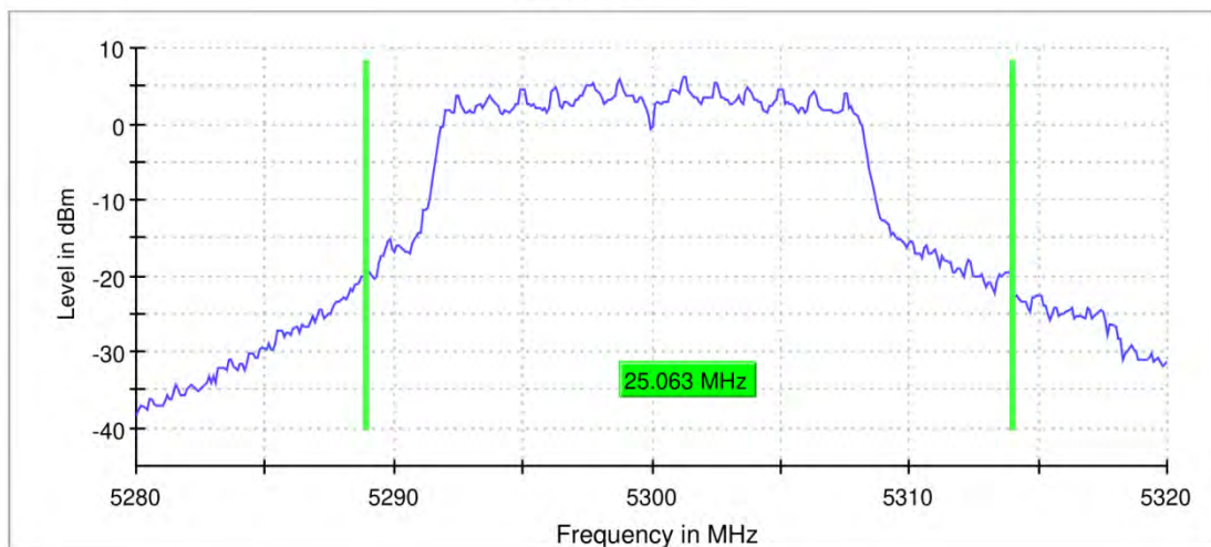
26 dB Bandwidth
