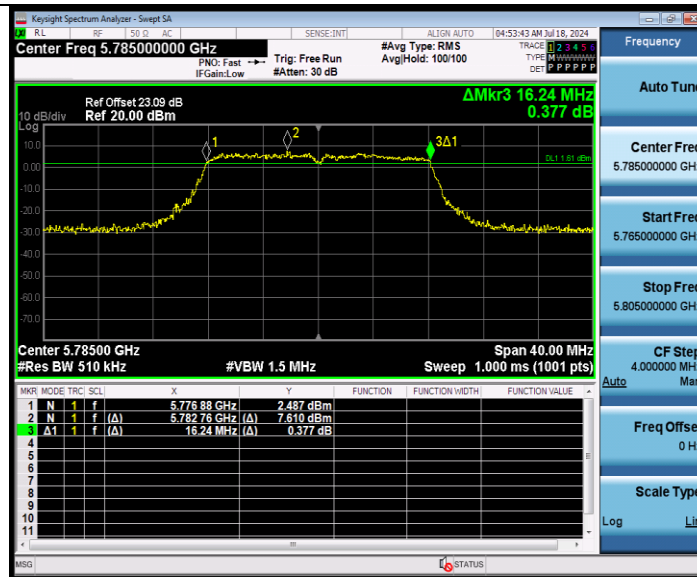
11A-CDD Ant2 5785
