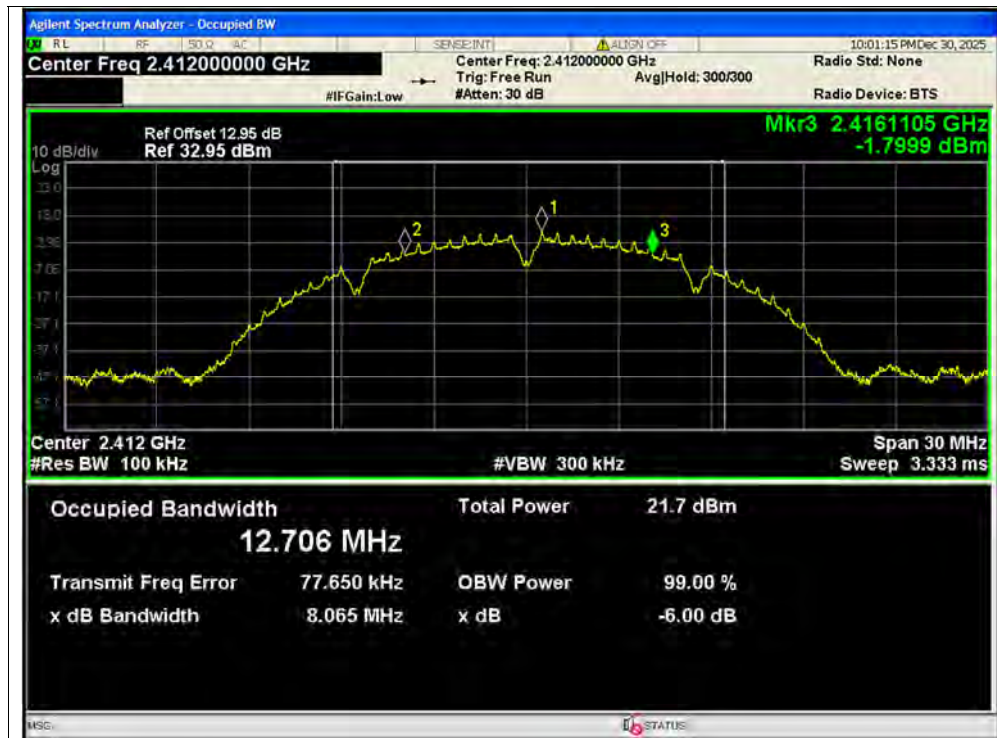
-6dB Bandwidth NVNT b 2412MHz Ant1
