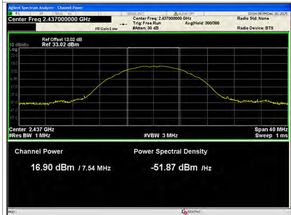
Peak Power NVNT b 2437MHz Ant1
