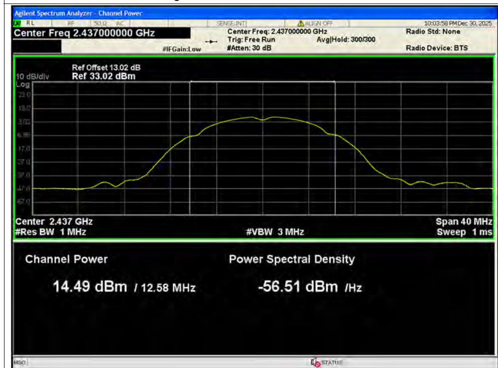
Average Power NVNT b 2437MHz Ant1
