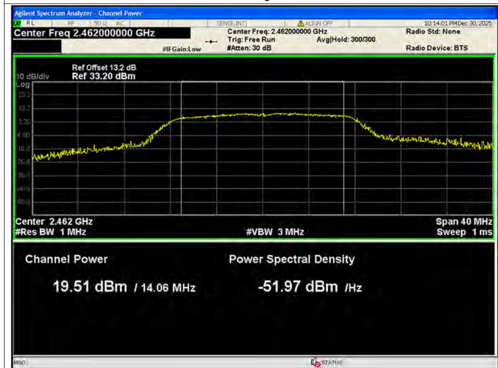
Peak Power NVNT g 2462MHz Ant1
