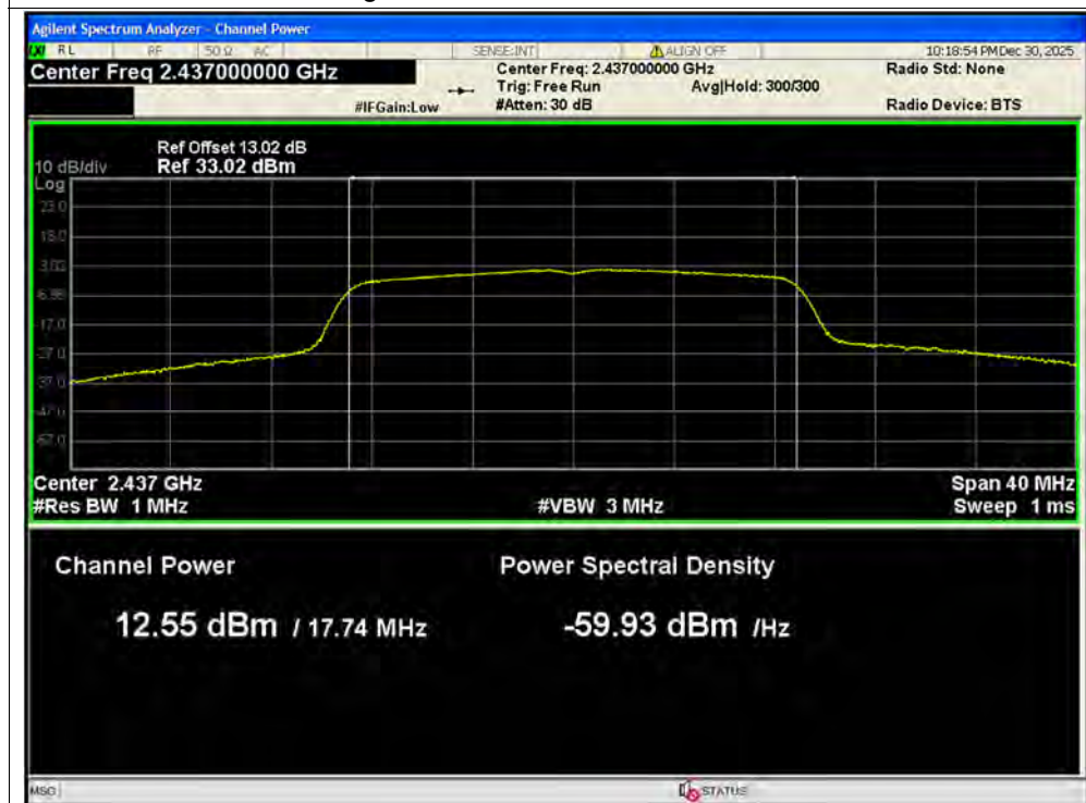
Average Power NVNT n20 2437MHz Ant1
