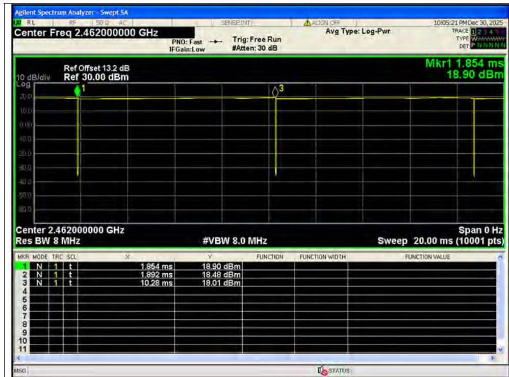
Duty Cycle NVNT b 2462MHz Ant1
