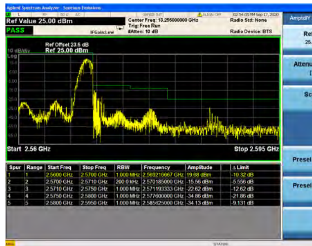
Band7 / 10MHz / High CH / QPSK / 1 RB
