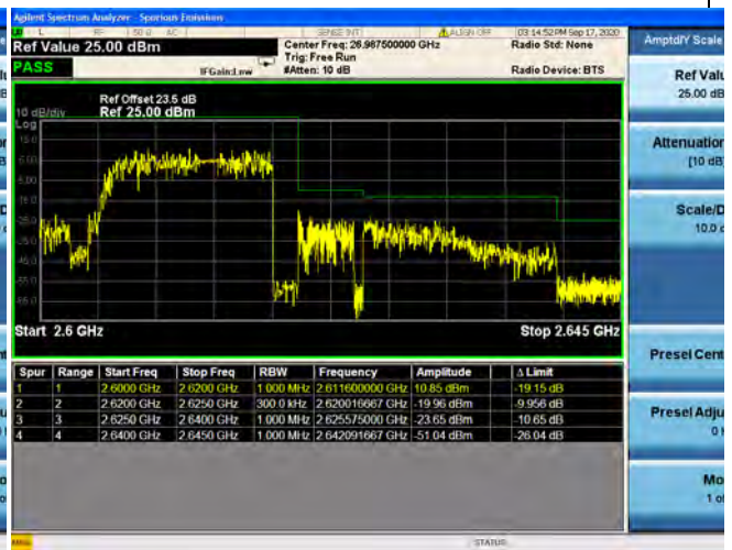
Band38 / 15MHz / High CH / QPSK / FULL RB
