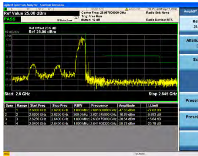
Band38 / 15MHz / High CH / QPSK / 1 RB
