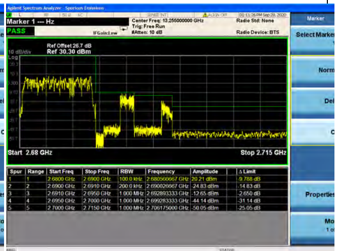
Band41 / 10MHz / High CH / QPSK / FULL RB
