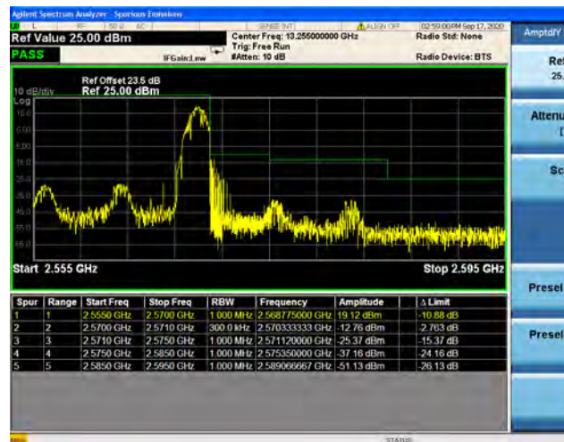
Band7 / 15MHz / High CH / QPSK / 1 RB
