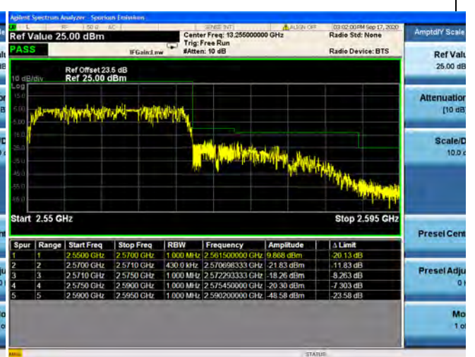
Band7 / 20MHz / High CH / QPSK / FULL RB
