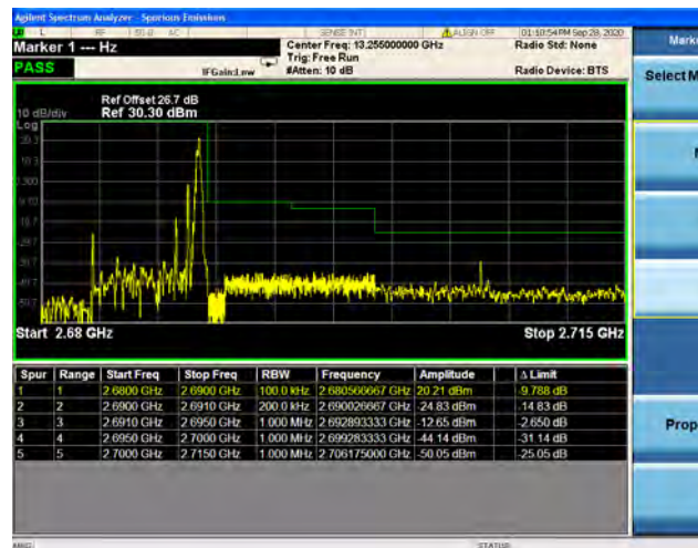
Band41 / 10MHz / High CH / QPSK / 1 RB
