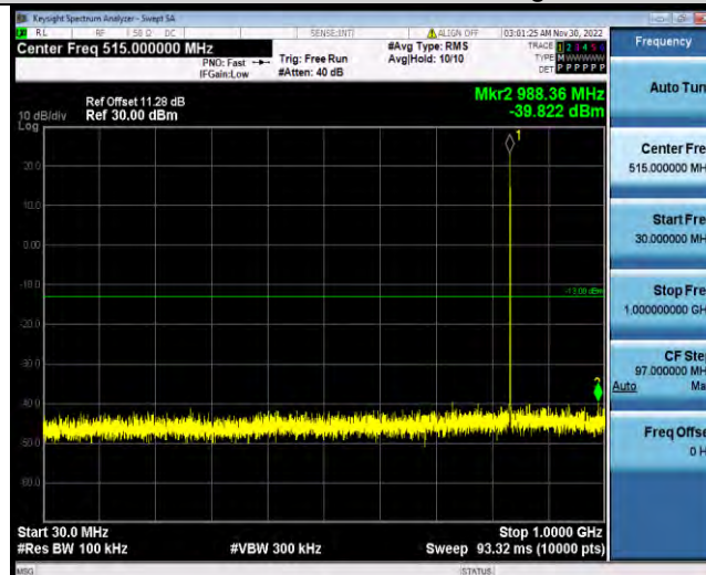
Band26-1.4MHz-QPSK-26915-1RB#0-Range1:30~1000MHz
