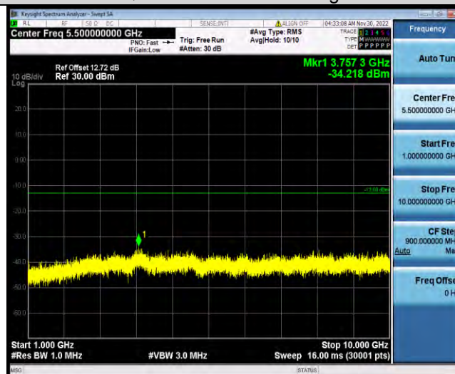
Band26-15MHz-64QAM-26965-1RB#0-Range2:1000~10000MHz
