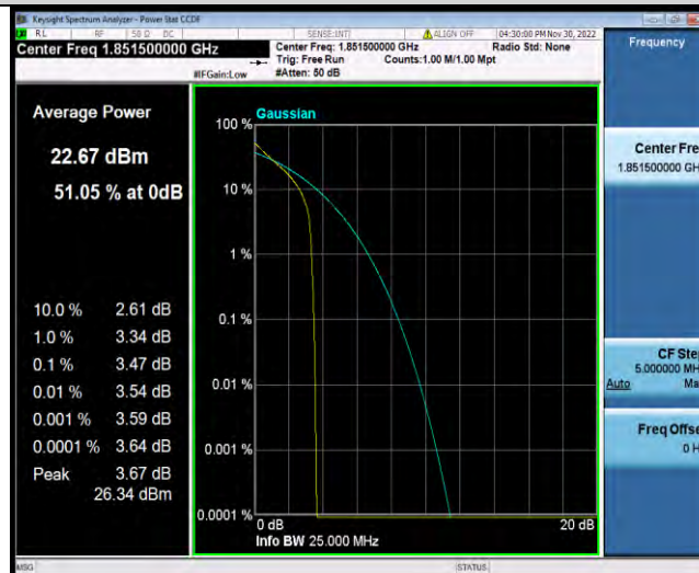
Band25-3MHz-QPSK-26055-15RB#0
