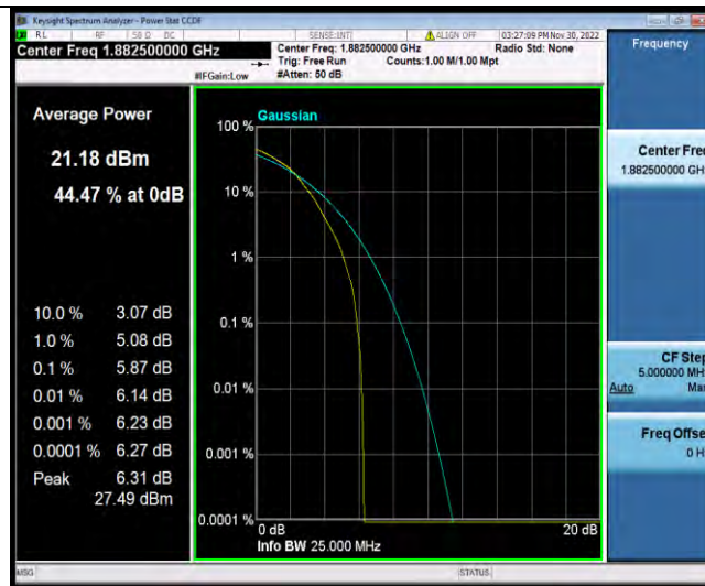
Band25-1.4MHz-64QAM-26365-6RB#0
