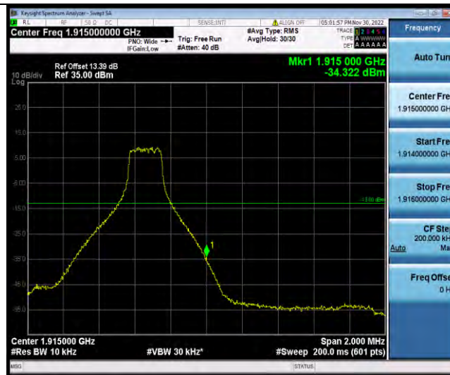
Band25-5MHz-64QAM-26665-25RB#0
