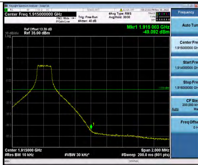
Band25-10MHz-64QAM-26640-50RB#0
