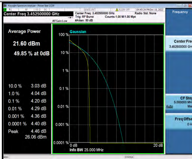
Band42-5MHz-QPSK-42115-25RB#0
