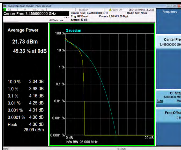
Band42-10MHz-QPSK-42140-50RB#0
