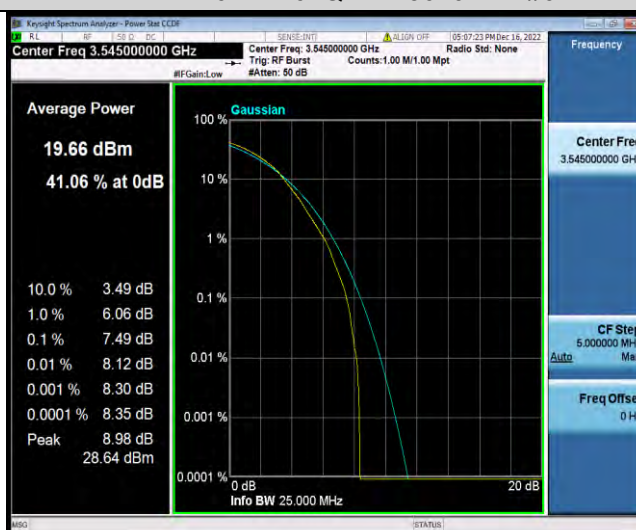
Band42-10MHz-64QAM-43040-50RB#0
