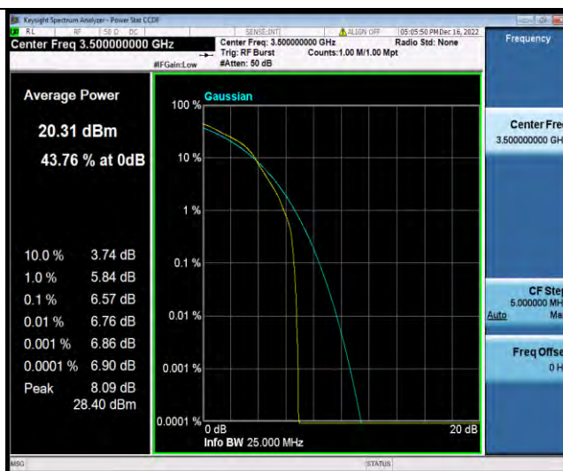
Band42-10MHz-16QAM-42590-50RB#0
