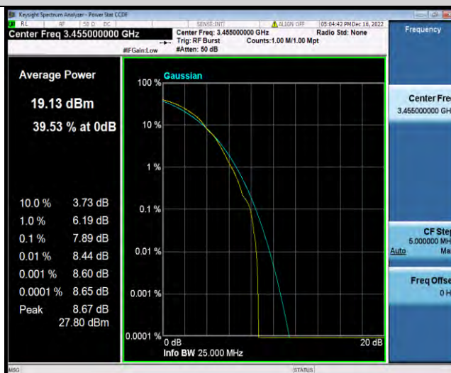
Band42-10MHz-64QAM-42140-50RB#0
