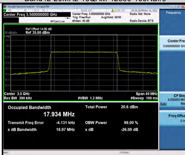
Band42-20MHz-16QAM-42990-100RB#0
