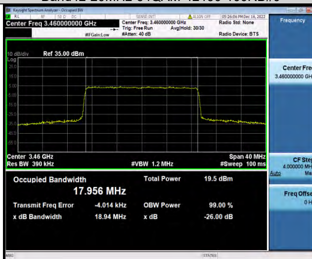
Band42-20MHz-64QAM-42590-100RB#0
