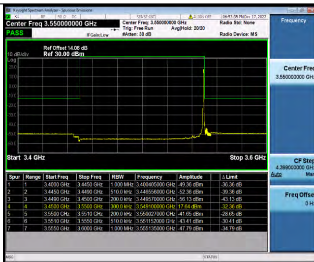
Band42-15MHz-QPSK-43015-75RB#0
