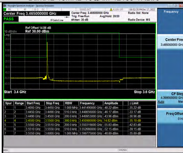
Band42-15MHz-16QAM-42165-75RB#0
