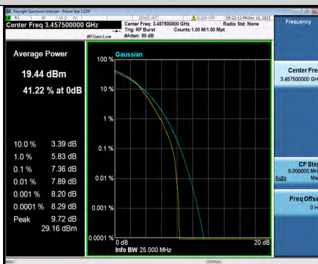
Band42-15MHz-64QAM-42165-75RB#0
