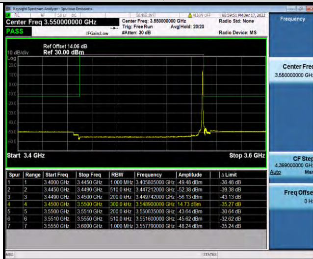
Band42-20MHz-16QAM-42990-100RB#0
