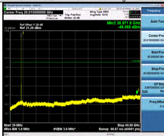
Band42-20MHz-16QAM-42590-1RB#0-Range1:30~40000MHz
