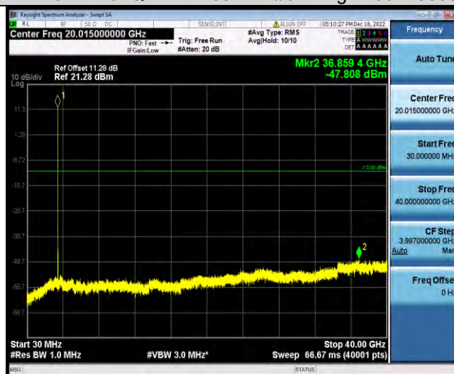
Band42-15MHz-64QAM-42590-1RB#0-Range1:30~40000MHz
