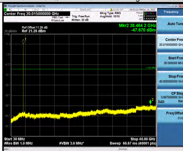
Band42-10MHz-64QAM-42590-1RB#0-Range1:30~40000MHz
