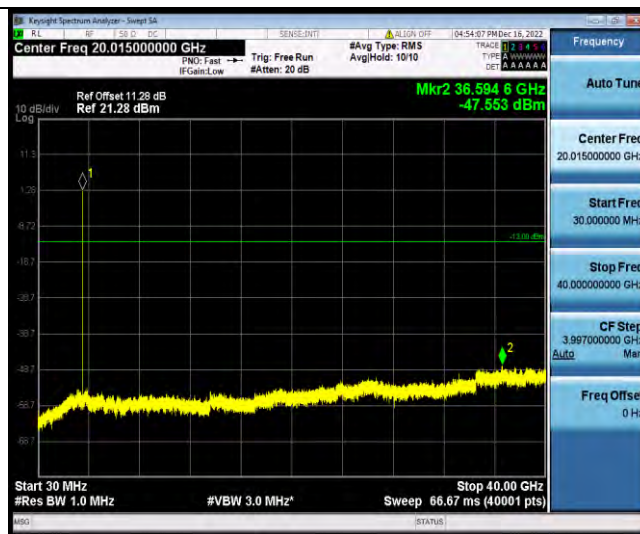
Band42-10MHz-16QAM-42140-1RB#0-Range1:30~40000MHz
