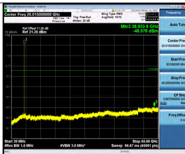
Band42-20MHz-16QAM-42190-1RB#0-Range1:30~40000MHz
