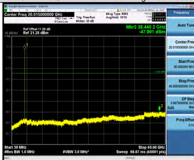
Band42-5MHz-16QAM-42590-1RB#0-Range1:30~40000MHz
