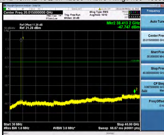
Band42-15MHz-16QAM-43015-1RB#0-Range1:30~40000MHz
