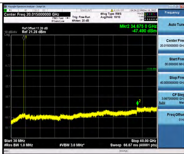
Band42-10MHz-64QAM-42140-1RB#0-Range1:30~40000MHz
