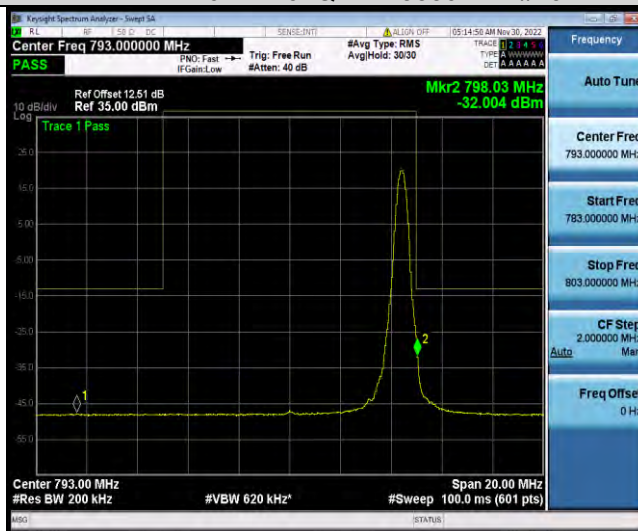
Band14-10MHz-64QAM-23330-50RB#0
