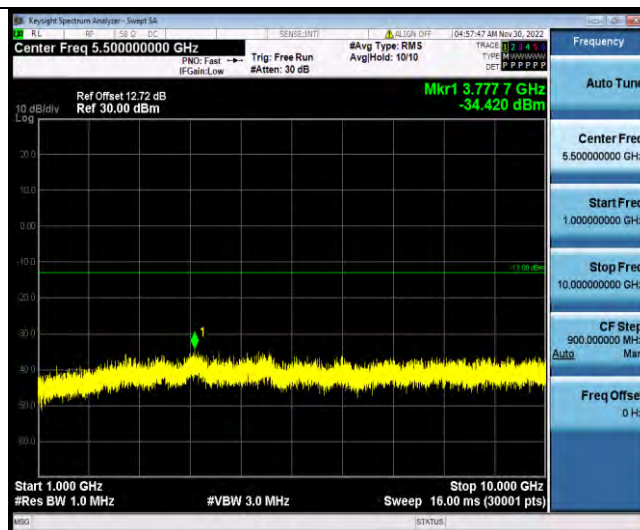
Band14-5MHz-QPSK-23330-1RB#0-Range3:1559~1610MHz
