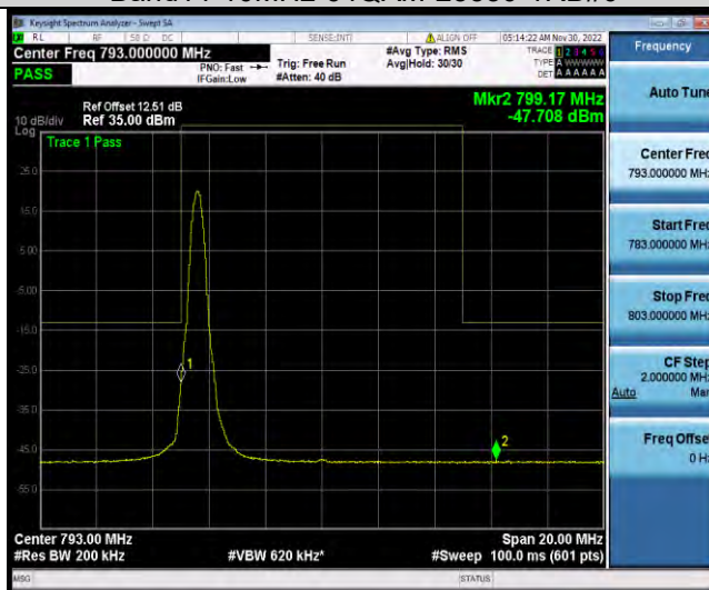
Band14-10MHz-64QAM-23330-1RB#49
