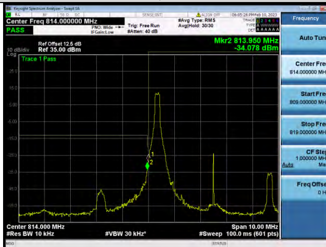
Band26-5MHz-QPSK-26715-25RB#0
