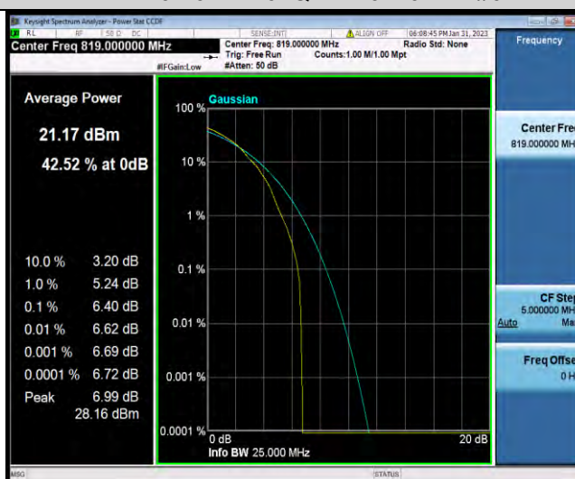
Band26-10MHz-64QAM-26740-50RB#0
