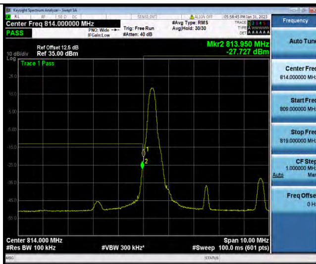
Band26-5MHz-64QAM-26715-25RB#0
