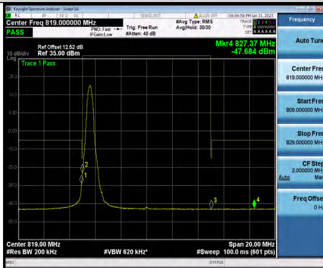
Band26-10MHz-64QAM-26740-1RB#49
