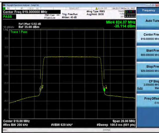
Band26-10MHz-64QAM-26740-1RB#0
