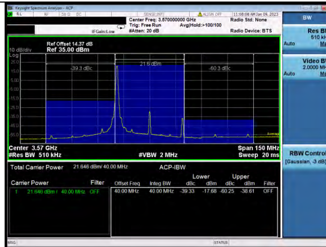
N48-40MHz-QPSK-638000-1RB#104
