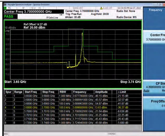
N48-10MHz-QPSK-646332-25RB#0
