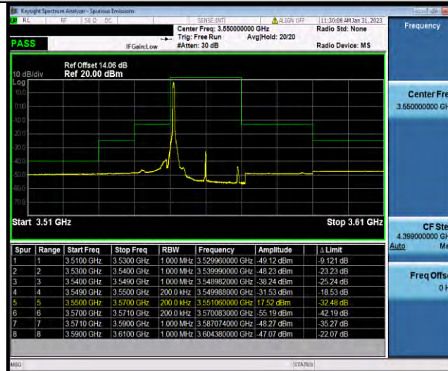
N48-20MHz-QPSK-637334-1RB#50
