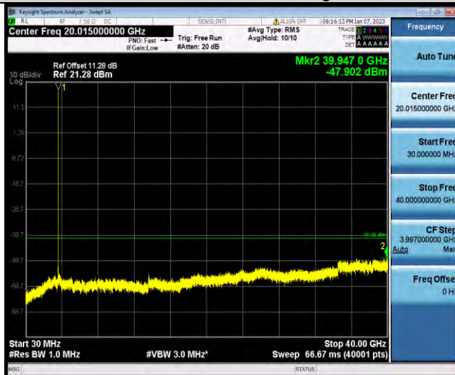
N48-10MHz-QPSK-646332-1RB#0-Range1:30~40000MHz
