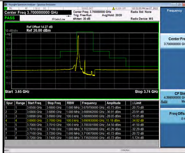
N48-10MHz-QPSK-646332-1RB#24
