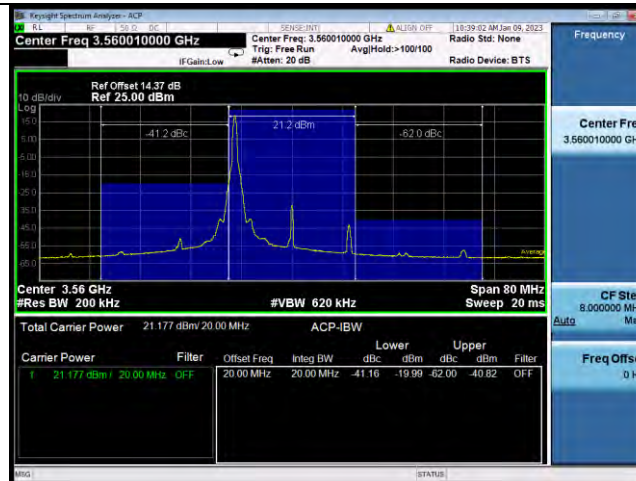
N48-20MHz-QPSK-637334-1RB#50
