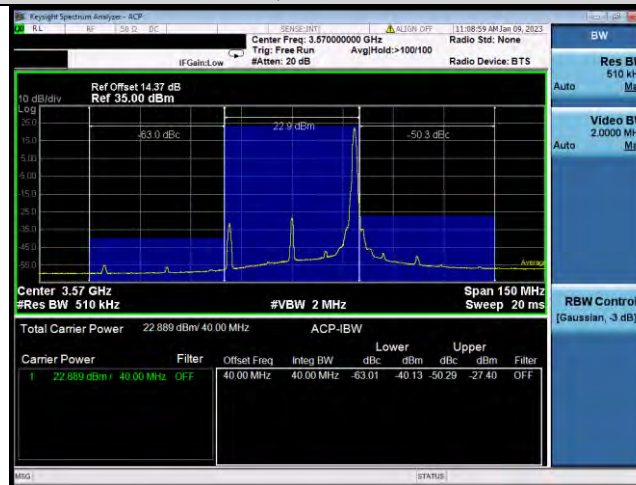
N48-40MHz-QPSK-638000-100RB#0
