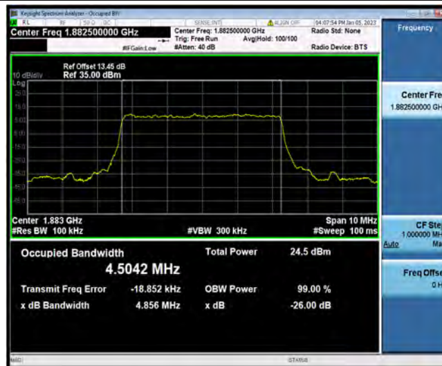
N25-5MHz-64QAM-376500-25RB#0
