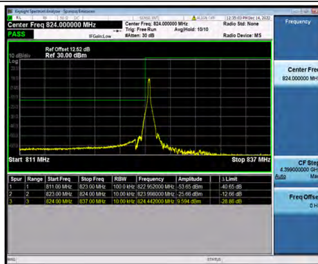
N5-10MHz-QPSK-165800-50RB#0
