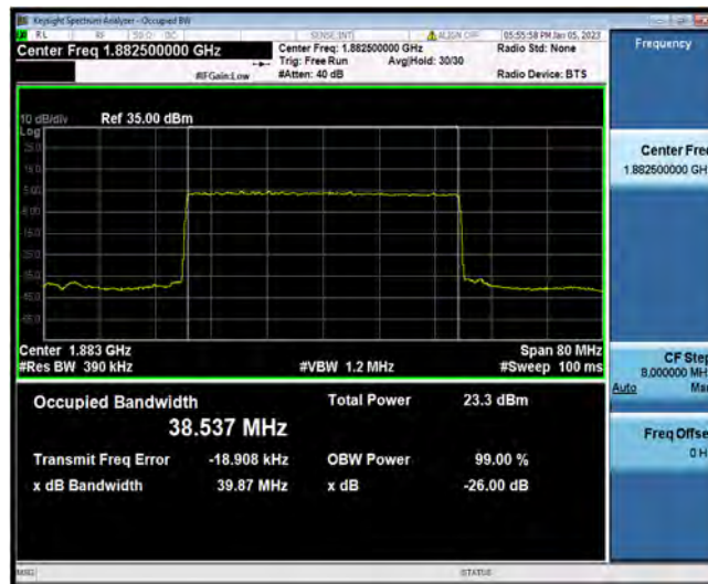
N25-40MHz-256QAM-376500-216RB#0
