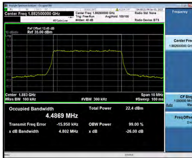
N25-5MHz-256QAM-376500-25RB#0
