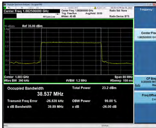
N25-40MHz-16QAM-376500-216RB#0
