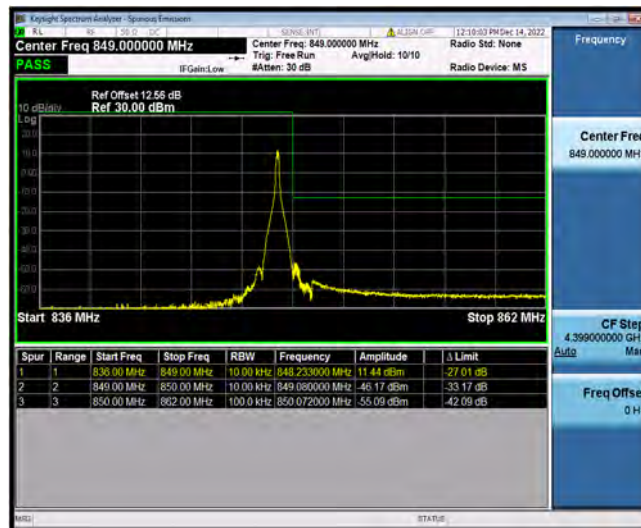
N5-10MHz-QPSK-168800-50RB#0
