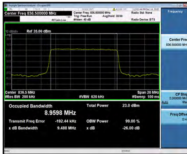
N5-10MHz-256QAM-167300-50RB#0
