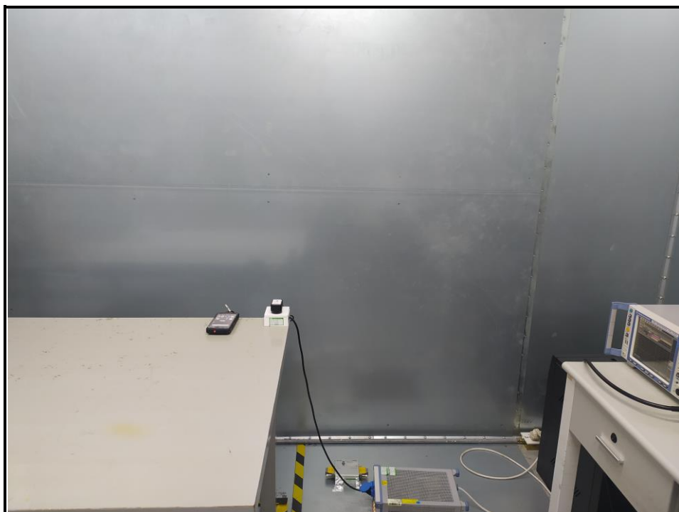
Fig. 3 Power line conducted emission setup photo
