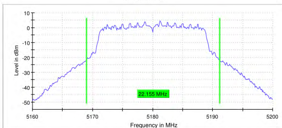
26 dB Bandwidth
