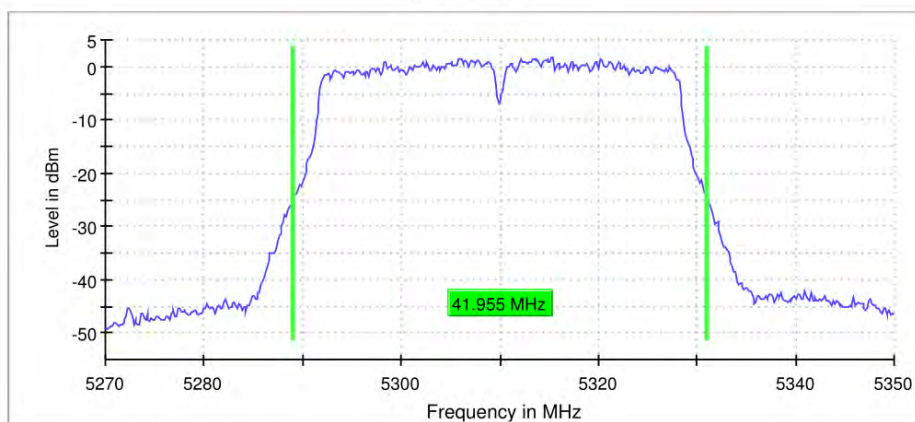
26 dB Bandwidth
