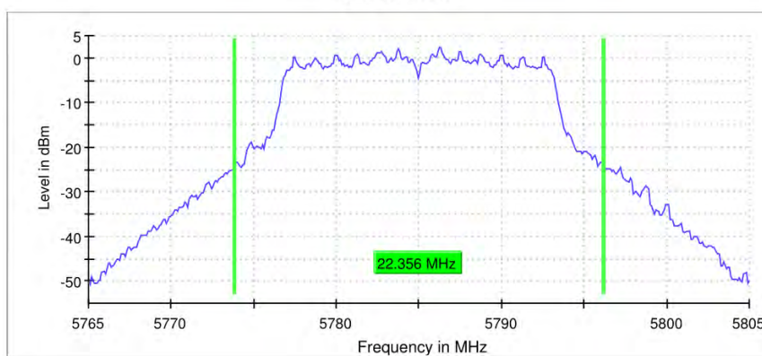
26 dB Bandwidth
