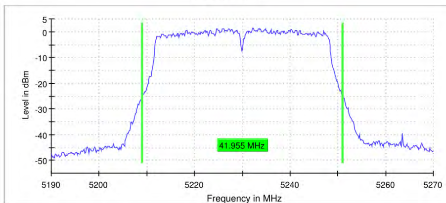
26 dB Bandwidth
