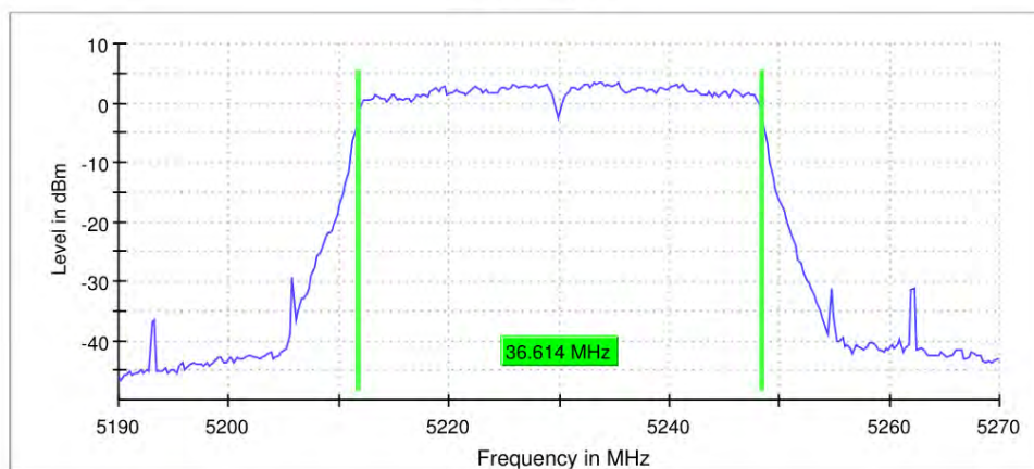
99 % Bandwidth
