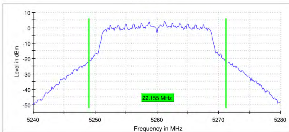
26 dB Bandwidth
