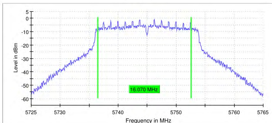
6 dB Bandwidth
