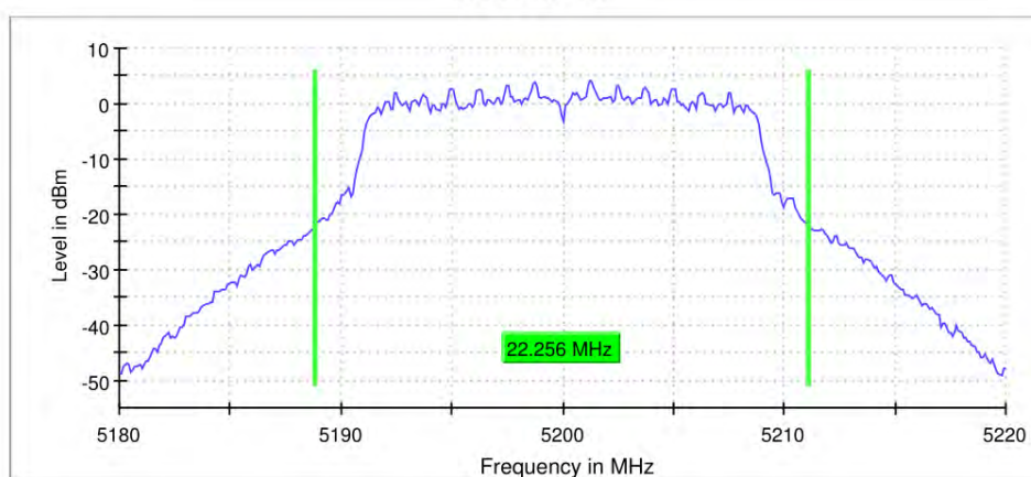
26 dB Bandwidth
