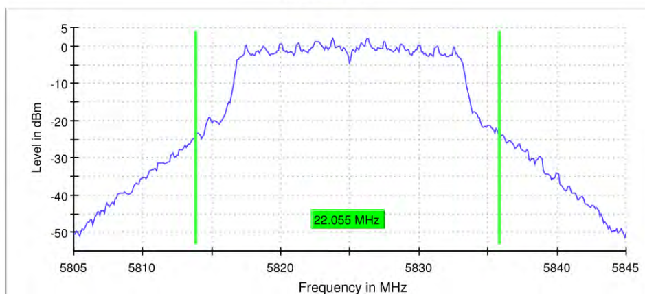
26 dB Bandwidth
