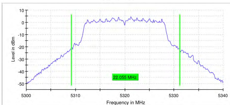
26 dB Bandwidth
