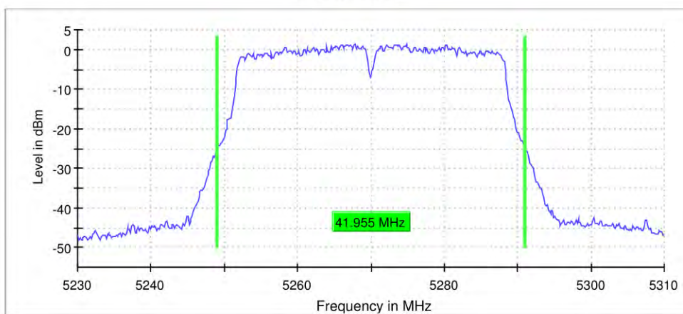
26 dB Bandwidth
