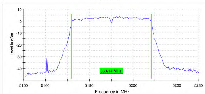
99 % Bandwidth
