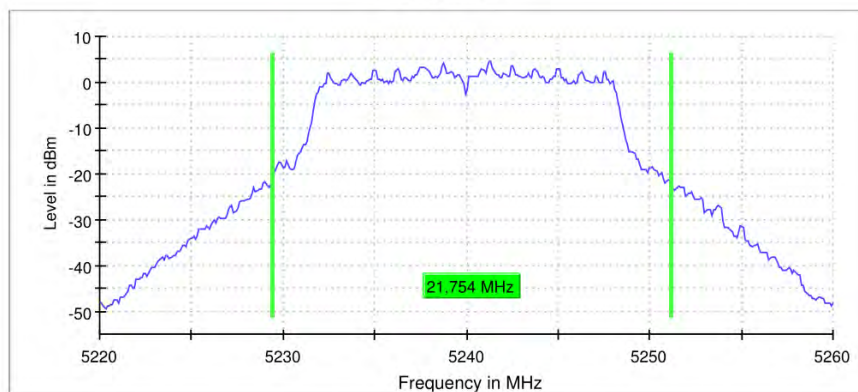
26 dB Bandwidth
