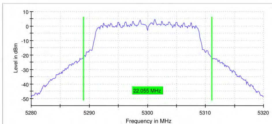
26 dB Bandwidth
