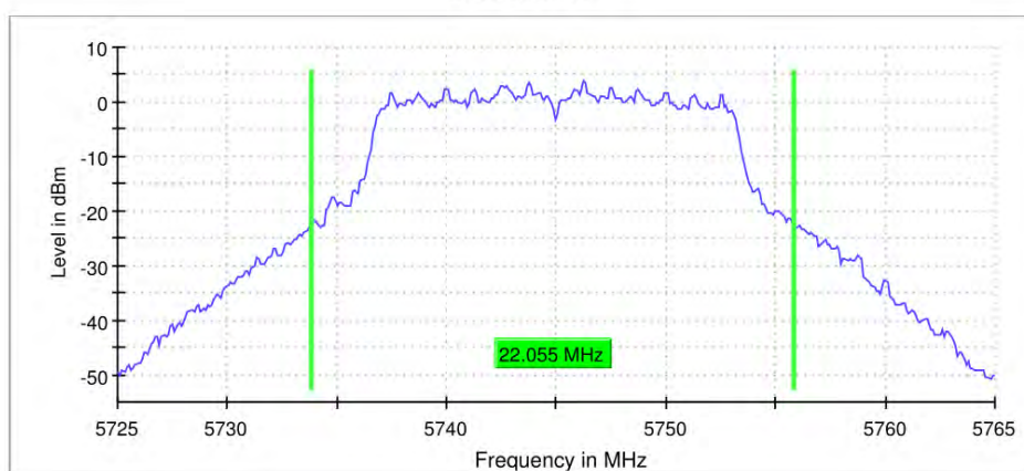
26 dB Bandwidth
