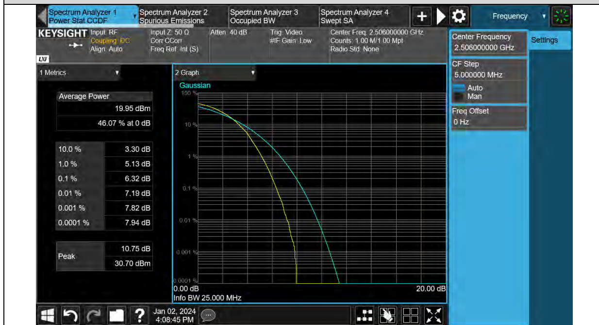
Band41-20MHz-64QAM-40620-1RB#0
