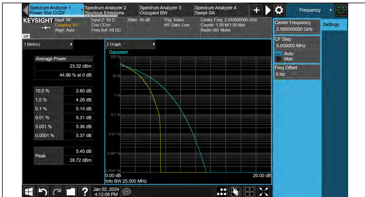
Band41-20MHz-QPSK-40620-100RB#0
