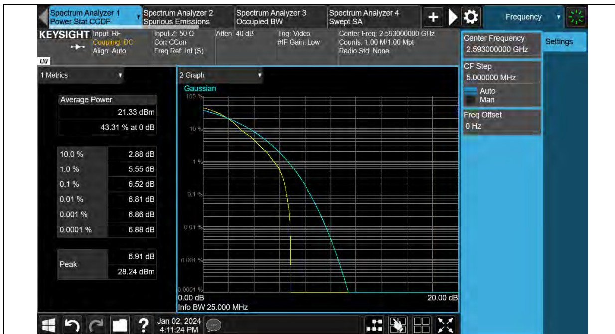
Band41-20MHz-64QAM-40620-100RB#0
