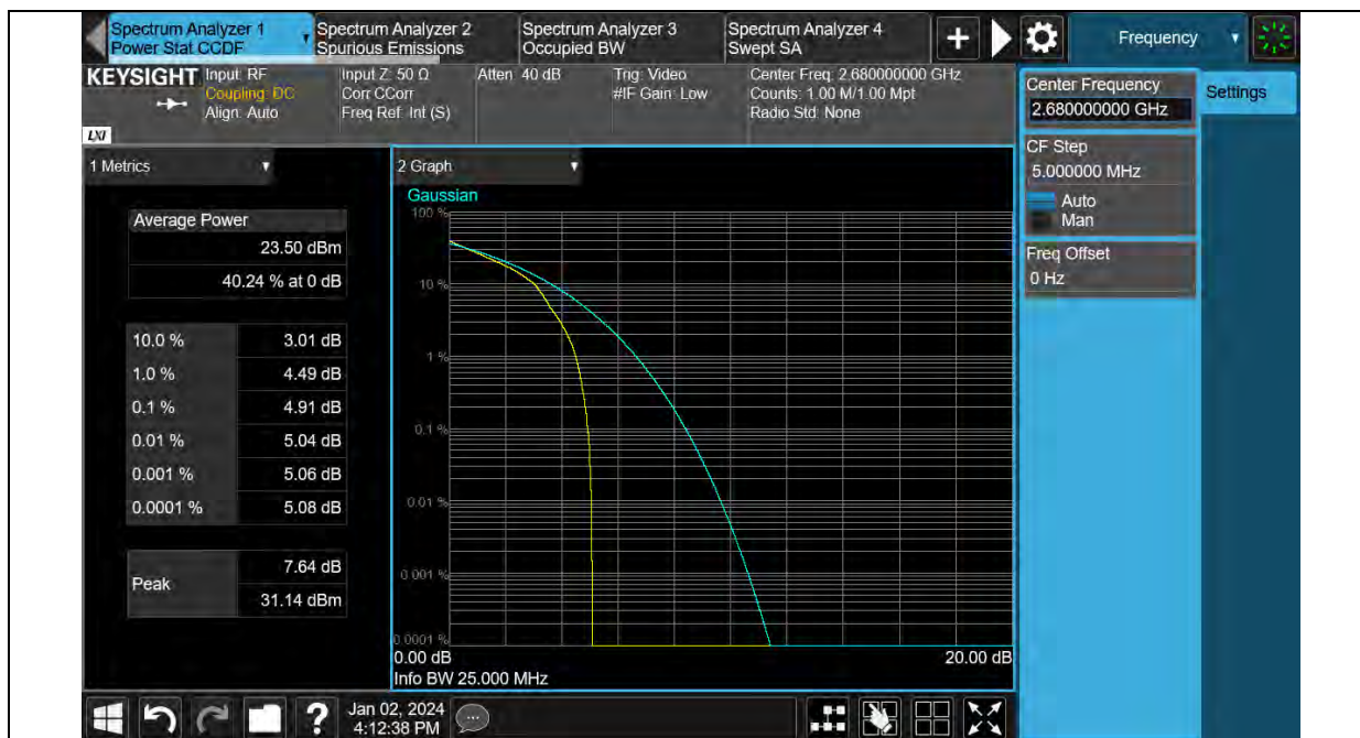
Band41-20MHz-QPSK-41490-100RB#0
