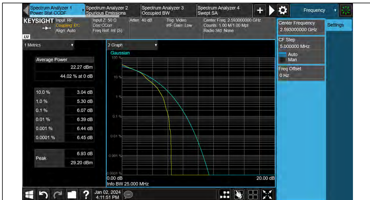
Band41-20MHz-16QAM-40620-100RB#0
