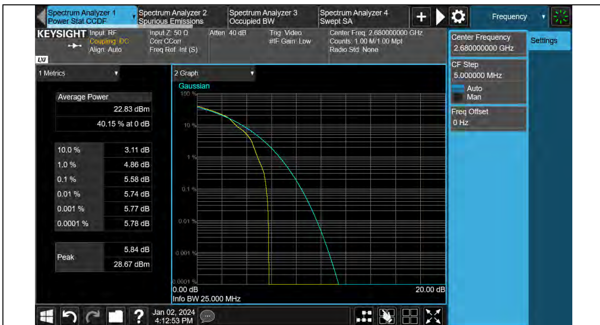
Band41-20MHz-16QAM-41490-100RB#0
