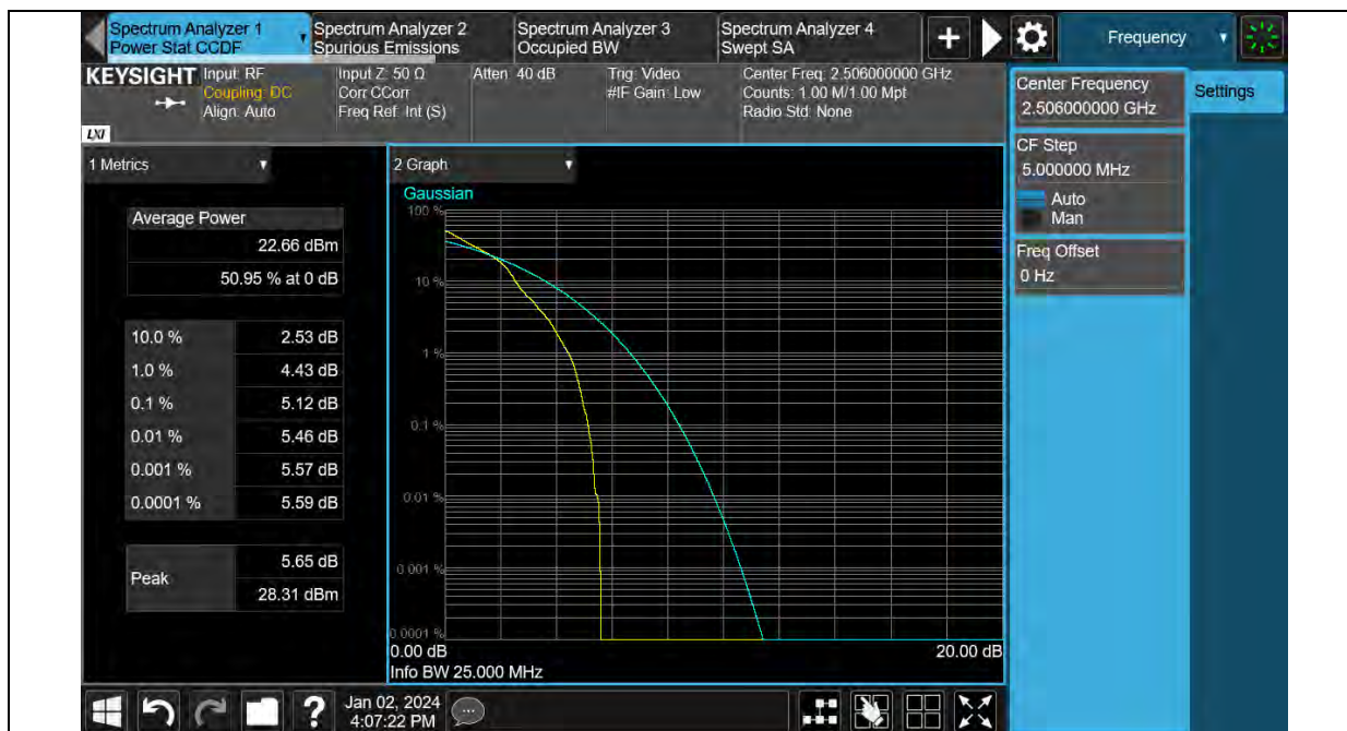
Band41-20MHz-16QAM-39750-100RB#0
