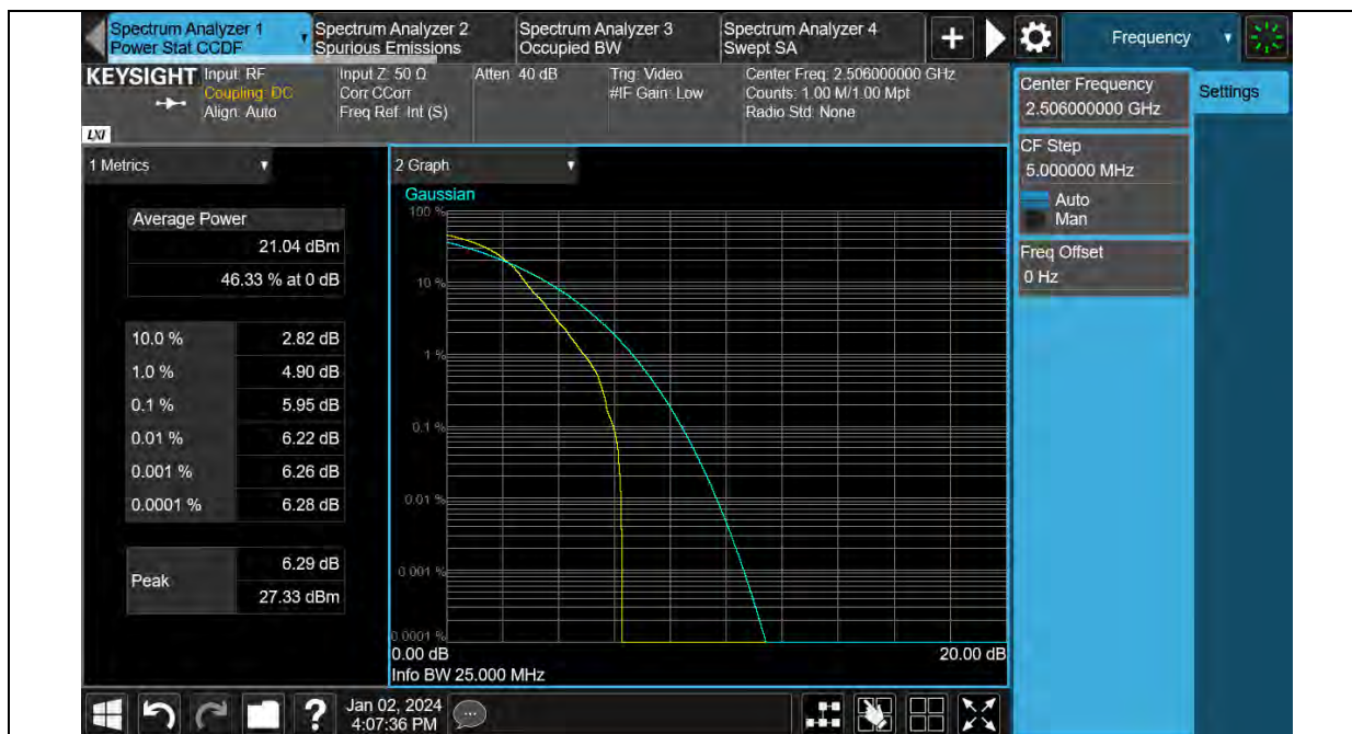
Band41-20MHz-64QAM-39750-100RB#0
