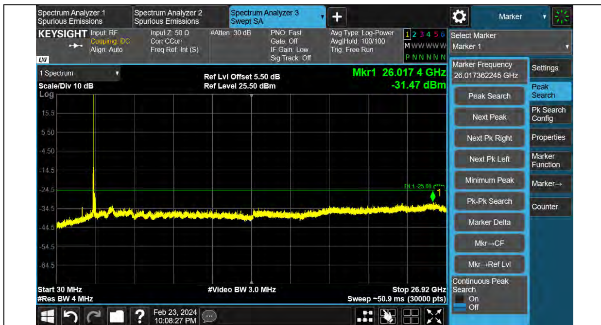
Band41-20MHz-QPSK-41490-1RB#0-Range:30~27000MHz
