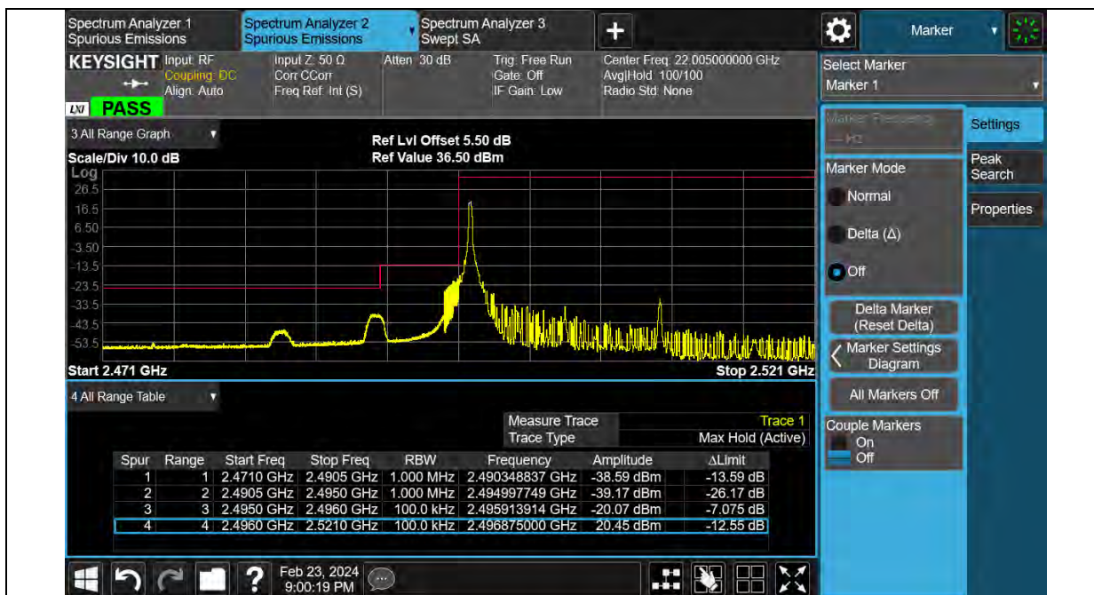
Band41-15MHz-16QAM-39725-75RB#0
