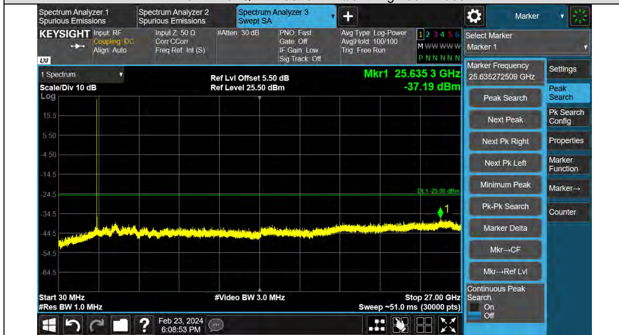
Band41-5MHz-64QAM-41565-1RB#0-Range:30~27000MHz
