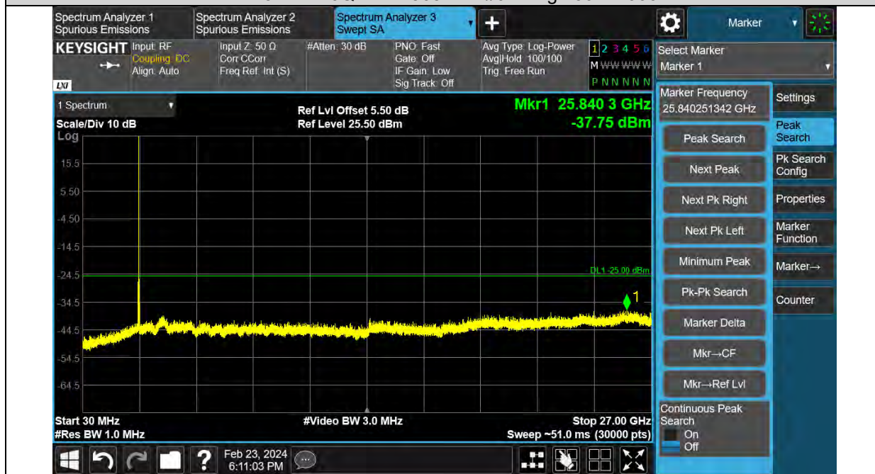
Band41-5MHz-64QAM-39675-1RB#0-Range:30~27000MHz
