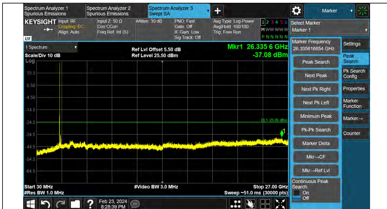
Band41-15MHz-64QAM-40620-1RB#0-Range:30~27000MHz
