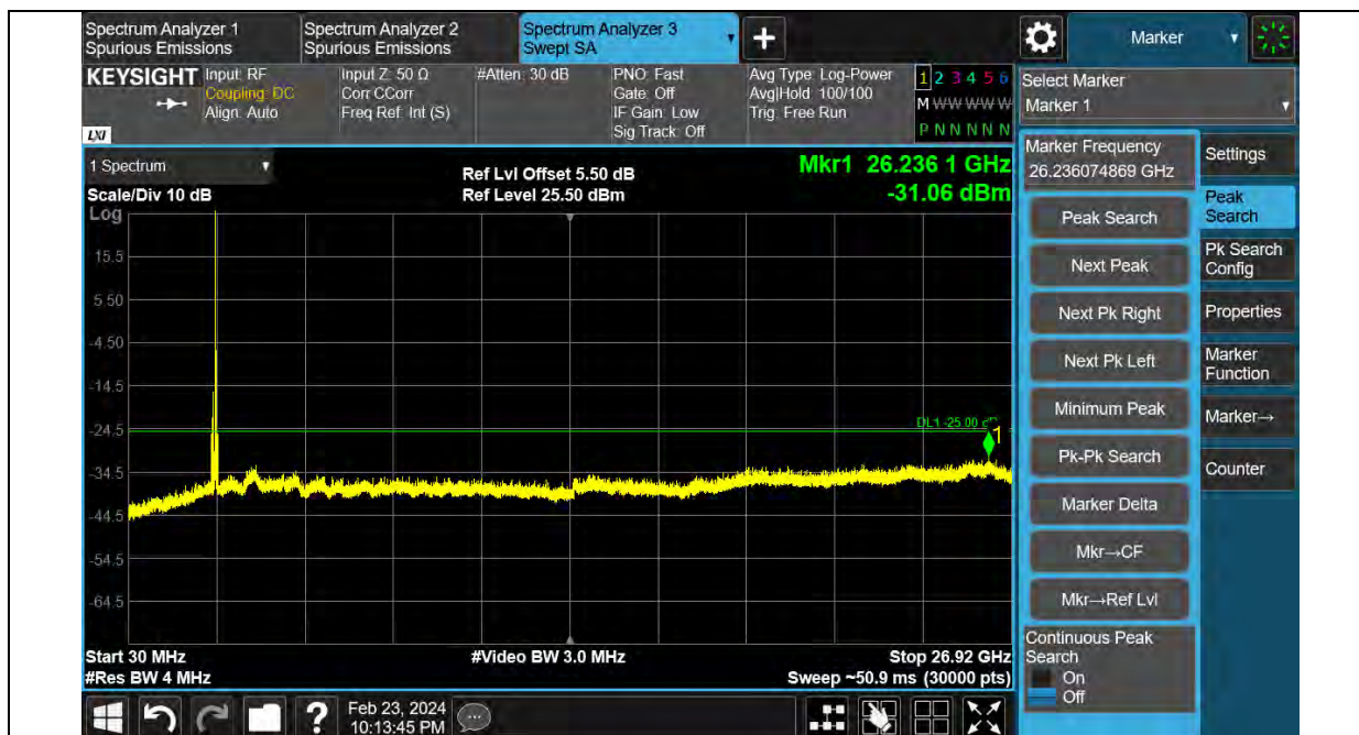
Band41-20MHz-64QAM-39750-1RB#0-Range:30~27000MHz
