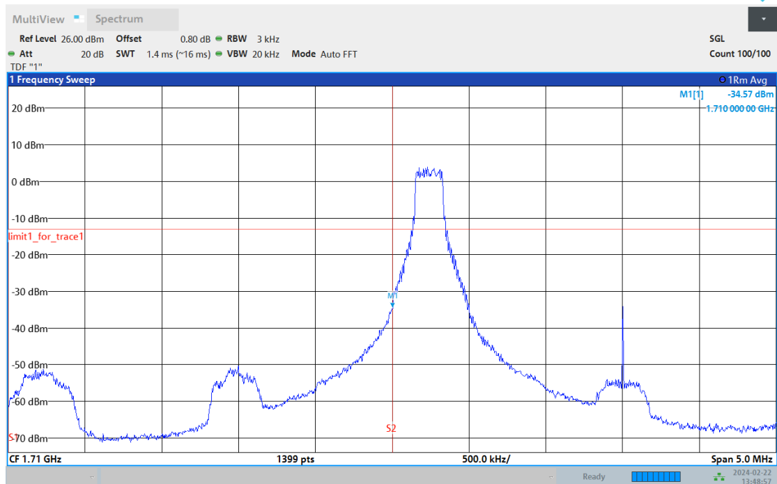
Band66-3MHz-64QAM-131987-15RB#0
