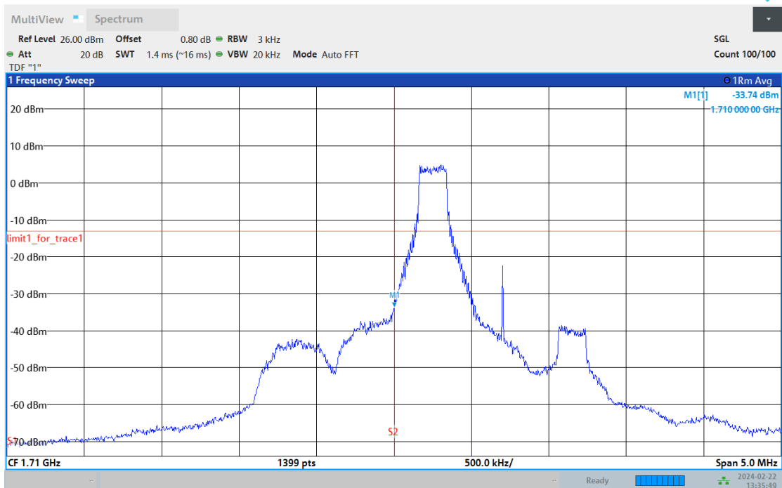
Band66-1.4MHz-16QAM-131979-6RB#0
