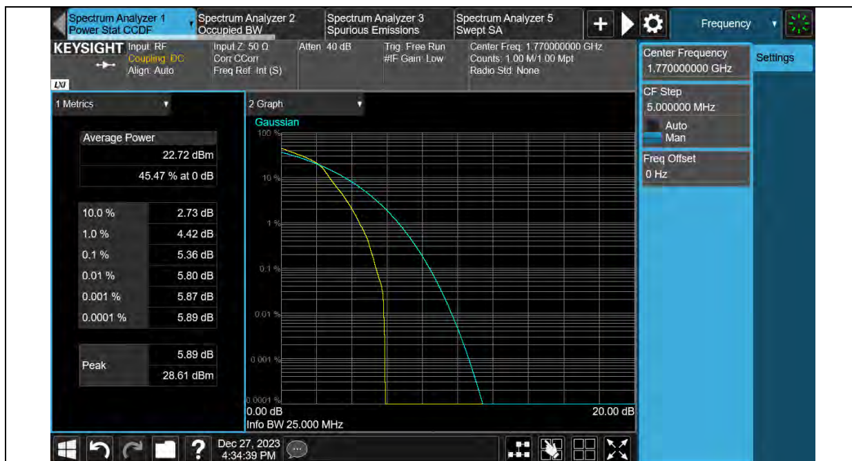
Band66-20MHz-16QAM-132572-100RB#0
