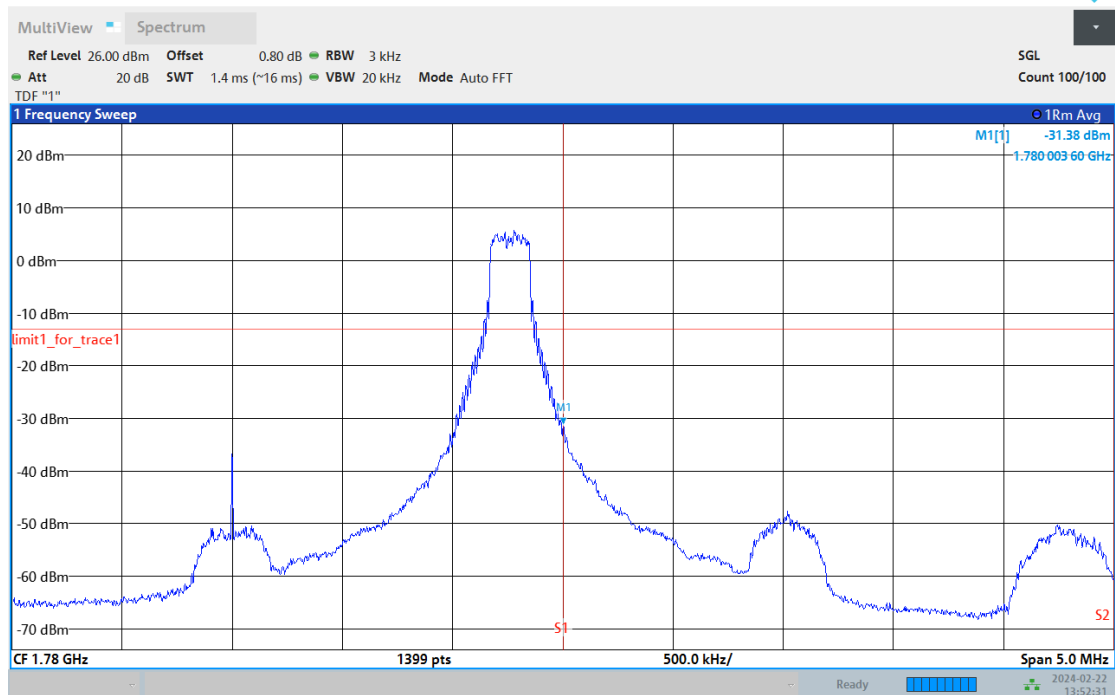
Band66-3MHz-16QAM-132657-15RB#0
