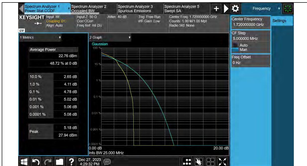
Band66-20MHz-16QAM-132072-100RB#0
