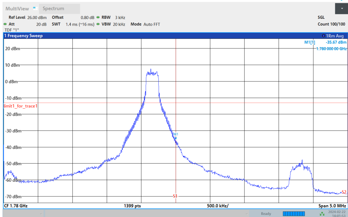
Band66-5MHz-QPSK-132647-25RB#0
