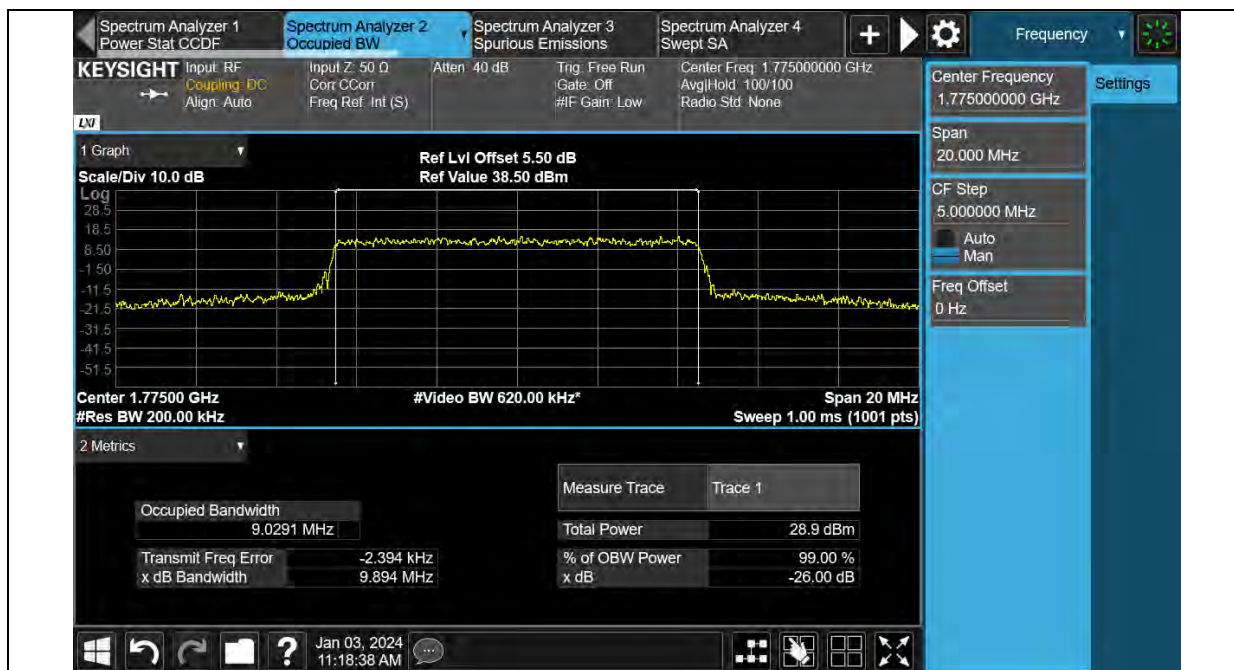
Band66-10MHz-64QAM-132022-50RB#0
