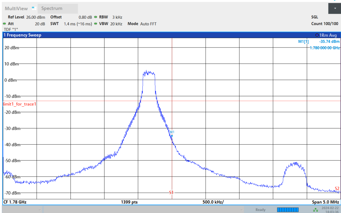
Band66-5MHz-16QAM-132647-25RB#0
