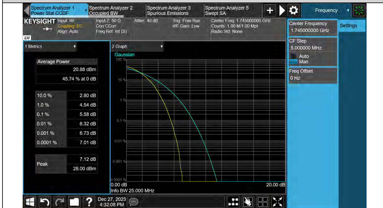
Band66-20MHz-64QAM-132572-1RB#0
