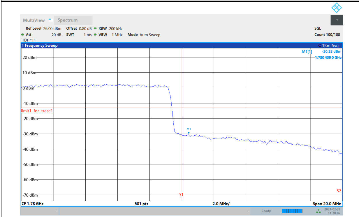
Band66-15MHz-64QAM-132597-75RB#0
