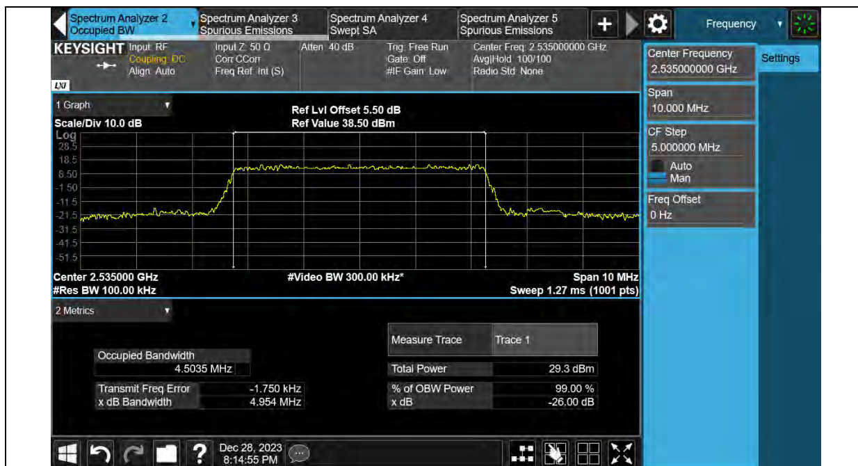
Band7-5MHz-16QAM-21425-25RB#0
