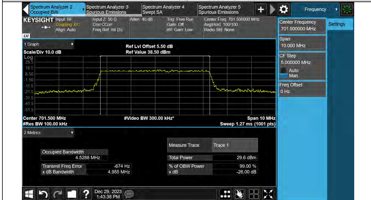
Band12-5MHz-16QAM-23095-25RB#0
