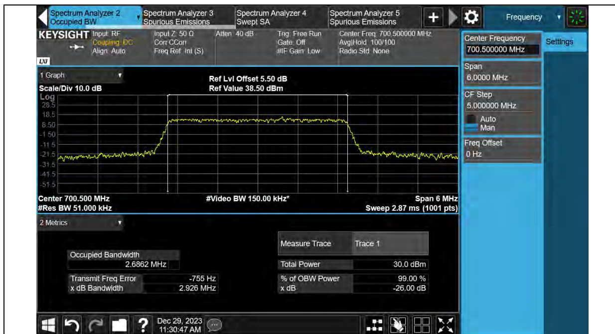
Band12-3MHz-16QAM-23095-15RB#0
