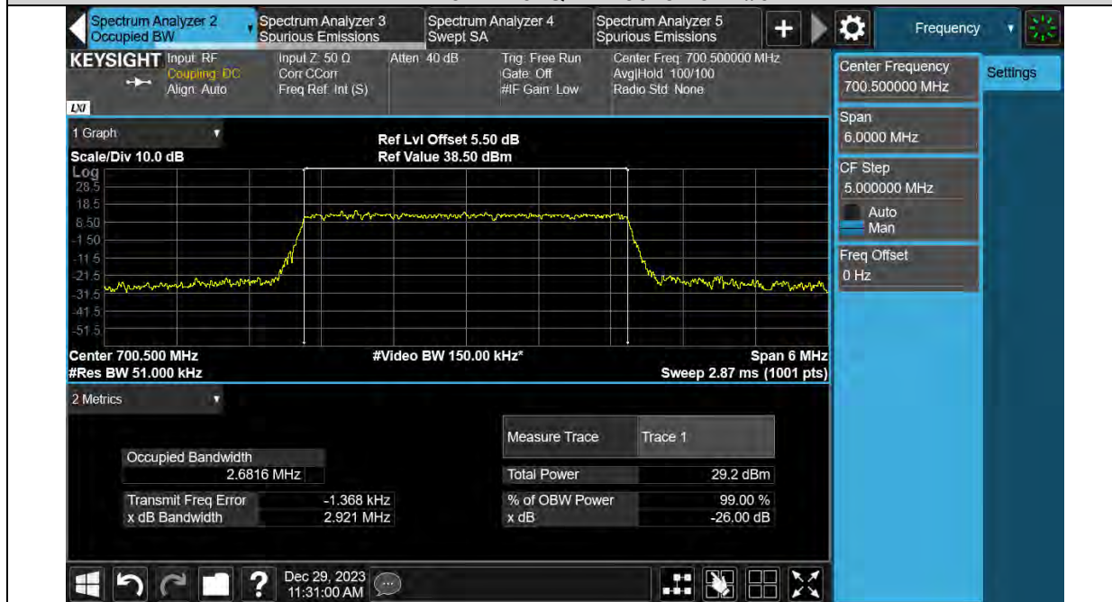
Band12-3MHz-64QAM-23095-15RB#0
