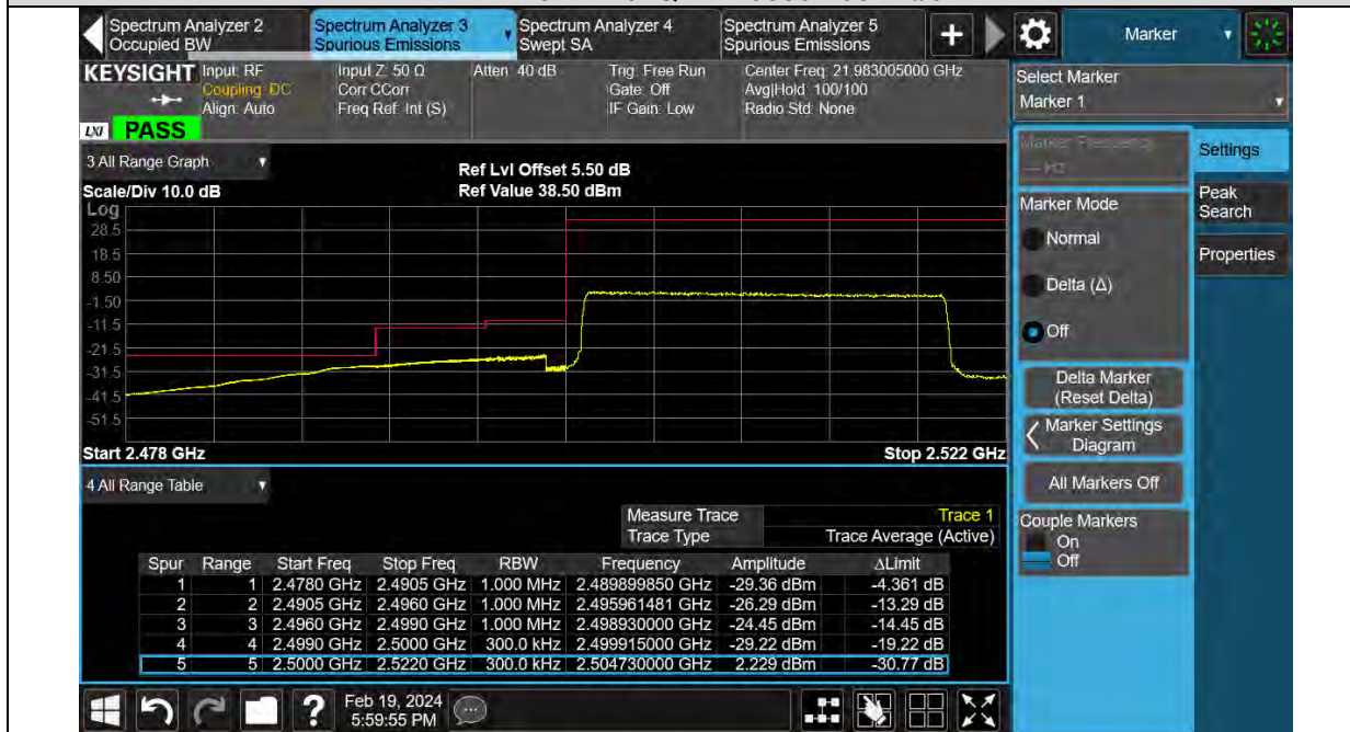
Band7-20MHz-64QAM-21350-1RB#99
