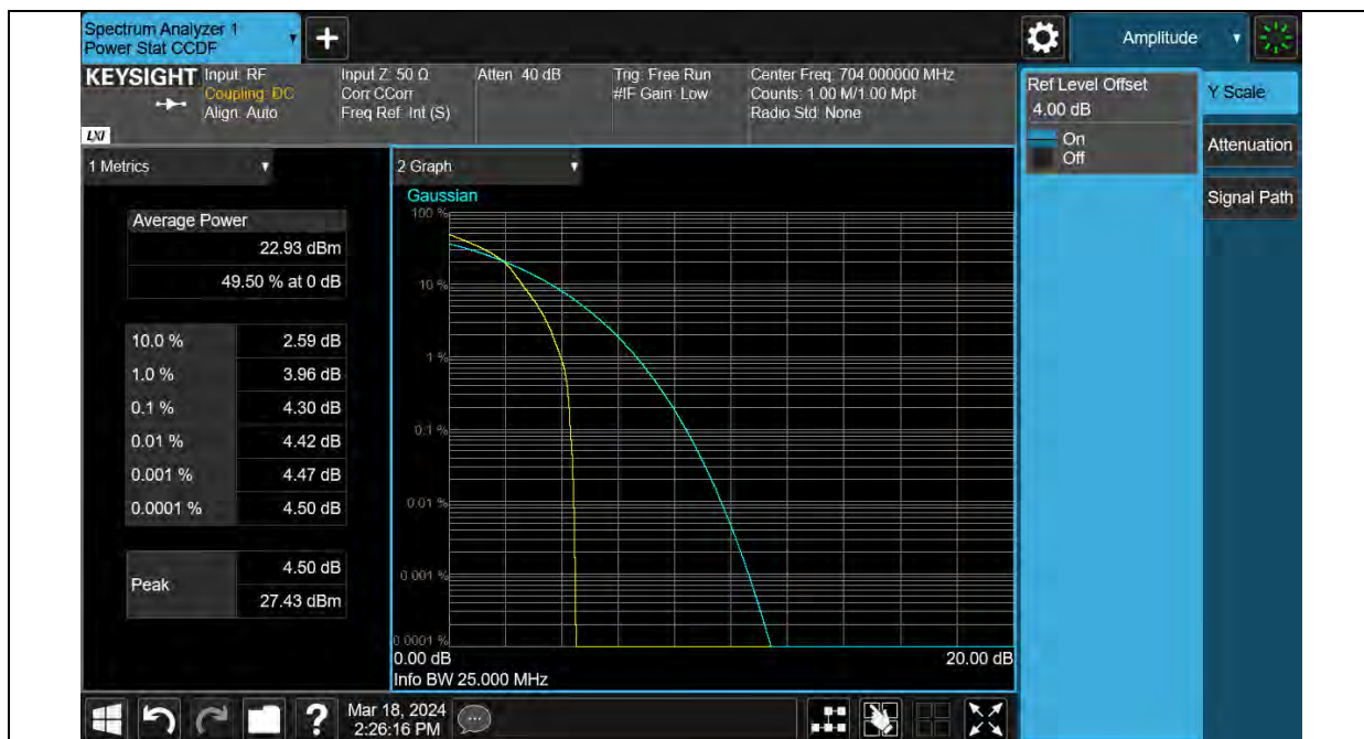
Band12-10MHz-16QAM-23060-50RB#0
