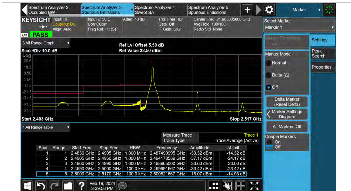
Band7-15MHz-16QAM-20825-75RB#0
