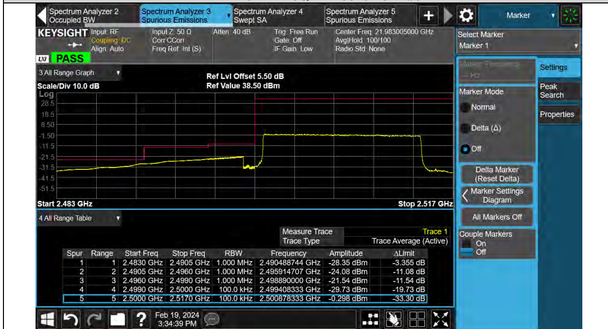
Band7-15MHz-16QAM-21375-1RB#74
