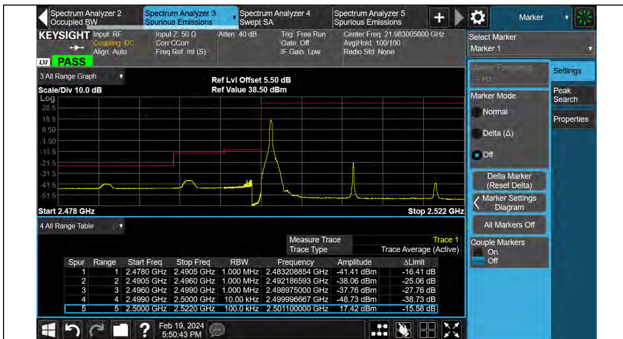
Band7-20MHz-64QAM-20850-100RB#0
