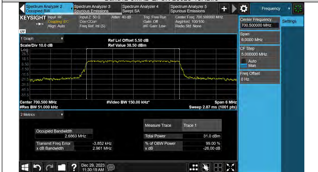
Band12-3MHz-QPSK-23095-15RB#0
