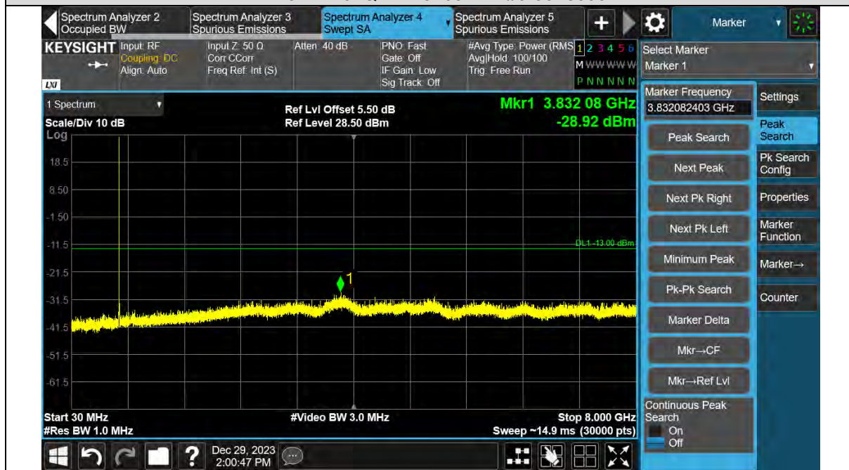
Band12-5MHz-QPSK-23035-1RB#0-30~8000MHz
