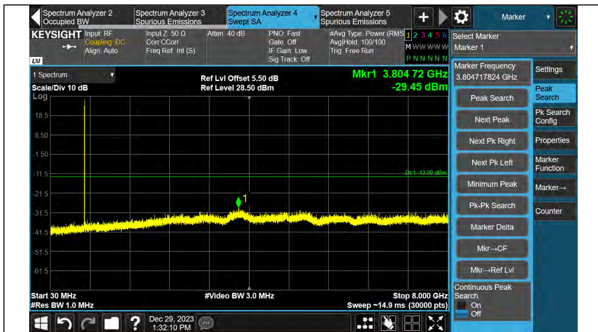
Band12-3MHz-64QAM-23025-1RB#0-30~8000MHz
