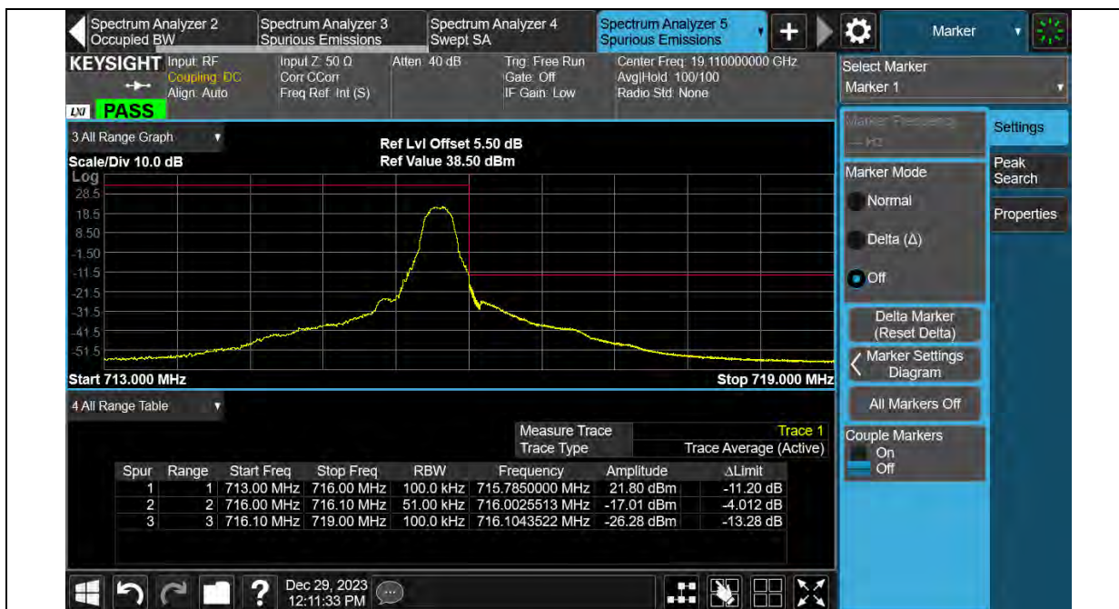
Band12-1.4MHz-QPSK-23173-6RB#0
