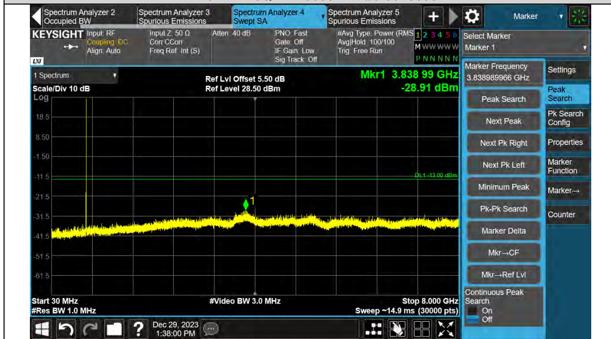
Band12-3MHz-16QAM-23165-1RB#0-30~8000MHz
