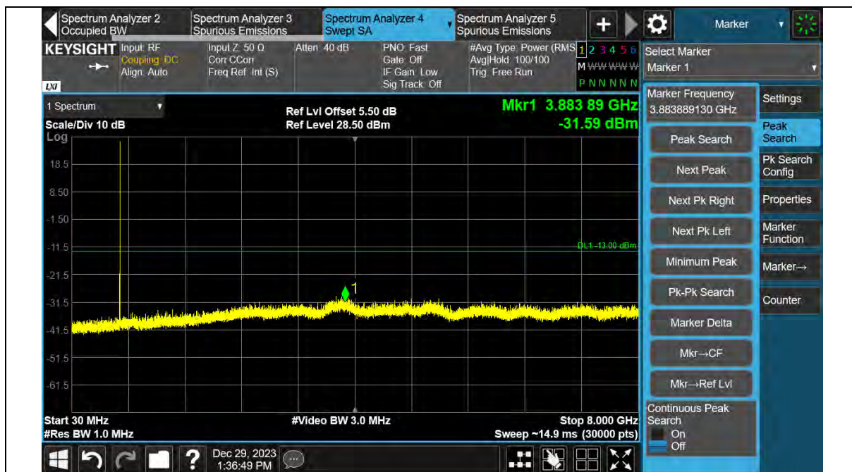
Band12-3MHz-64QAM-23165-1RB#0-30~8000MHz
