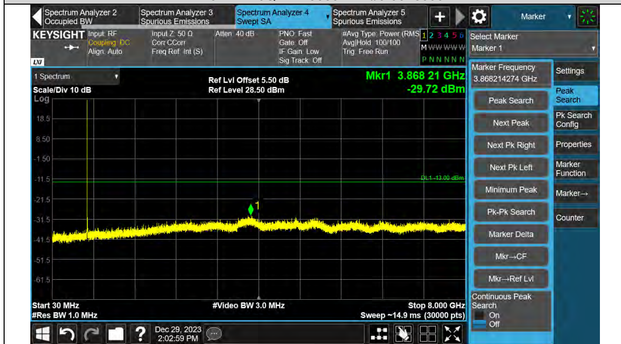
Band12-5MHz-16QAM-23095-1RB#0-30~8000MHz
