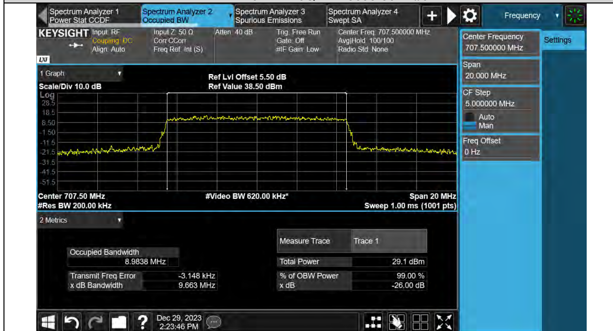
Band12-10MHz-16QAM-23130-50RB#0
