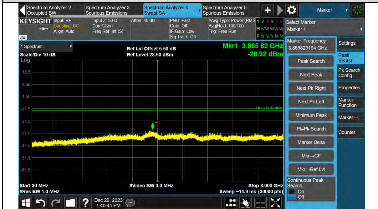
Band12-3MHz-64QAM-23095-1RB#0-30~8000MHz
