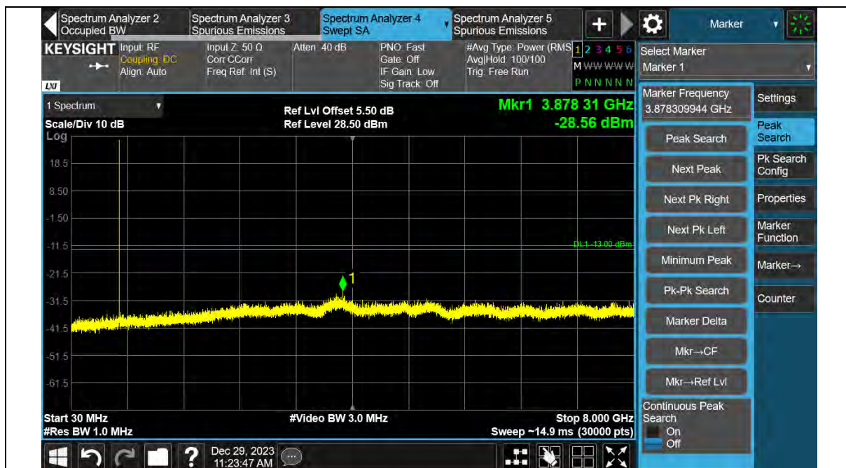
Band12-1.4MHz-16QAM-23173-1RB#0-30~8000MHz
