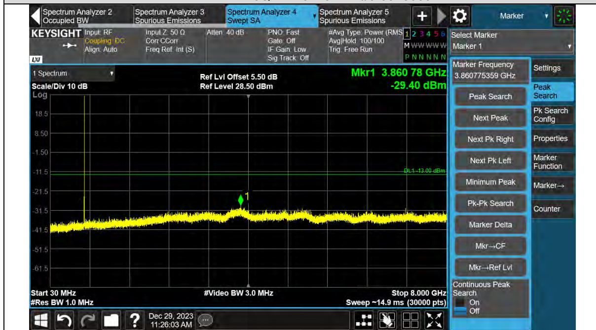
Band12-1.4MHz-64QAM-23017-1RB#0-30~8000MHz
