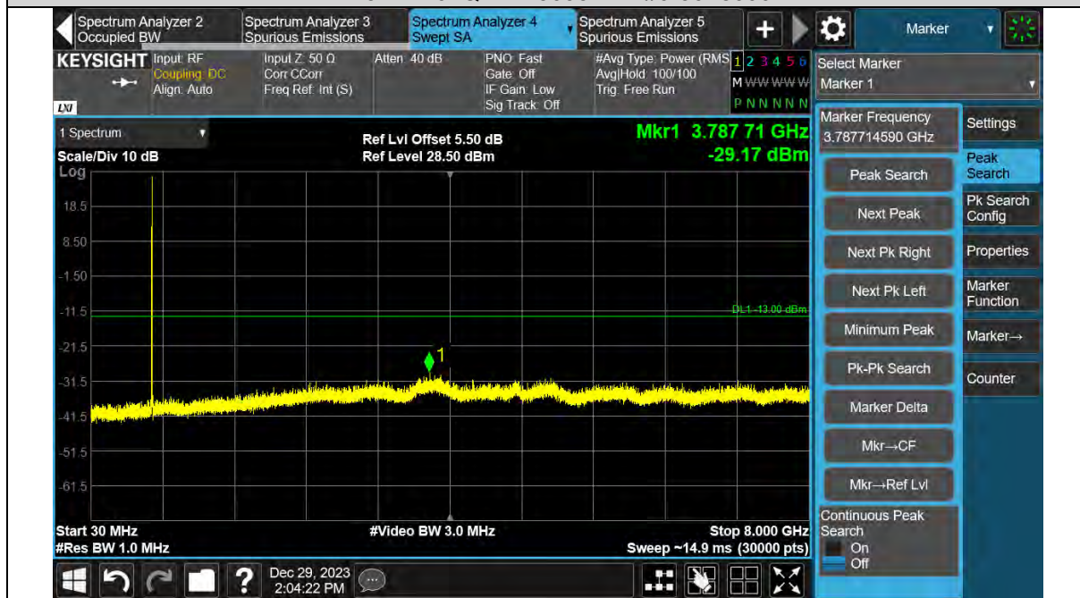
Band12-5MHz-64QAM-23155-1RB#0-30~8000MHz
