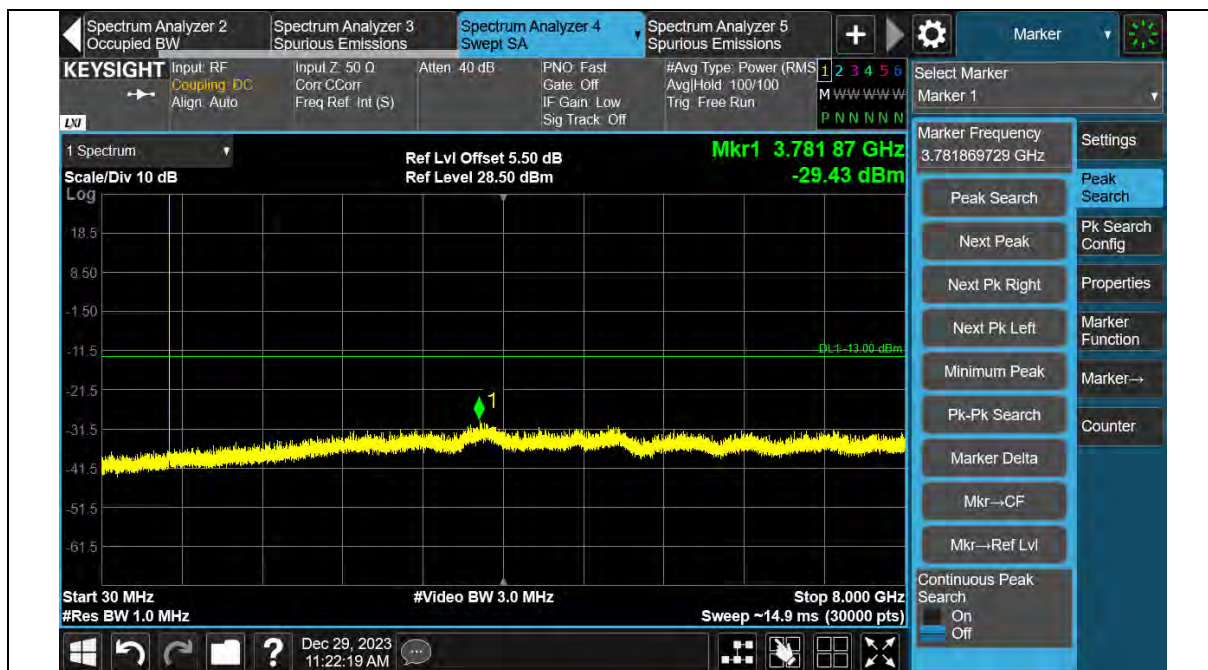
Band12-1.4MHz-64QAM-23095-1RB#0-30~8000MHz
