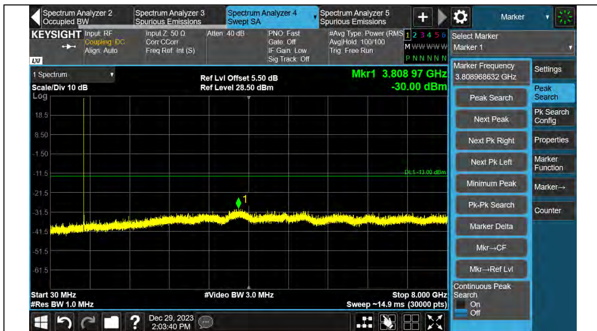
Band12-5MHz-64QAM-23095-1RB#0-30~8000MHz
