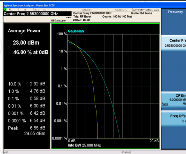
Band41-15MHz-16QAM-41515-1RB#0
