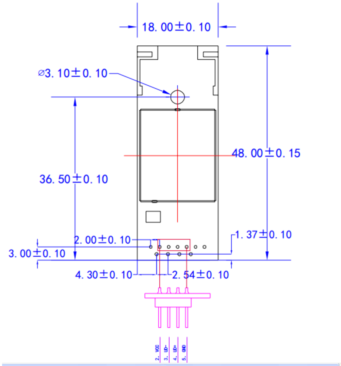
Figure 10: Bottom side 4-Pin 2.0mm pitch pin header interface.
