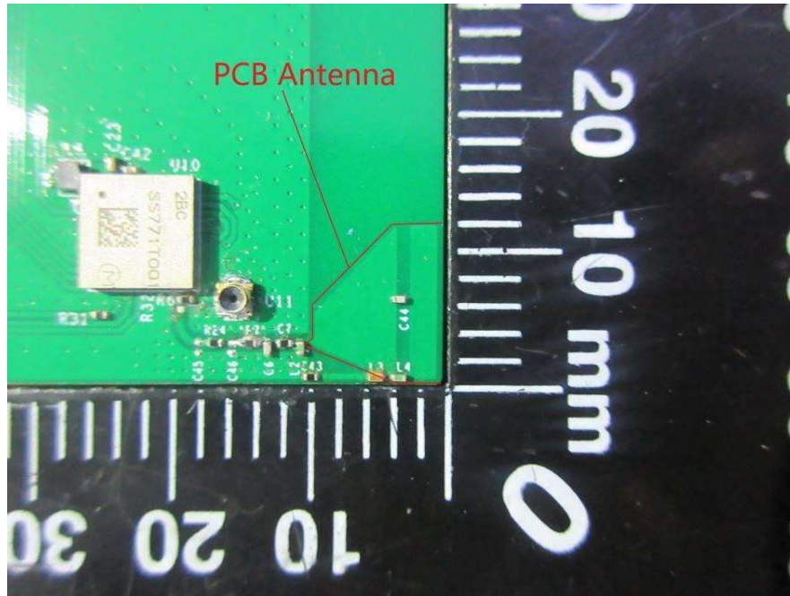
PCB Antenna
