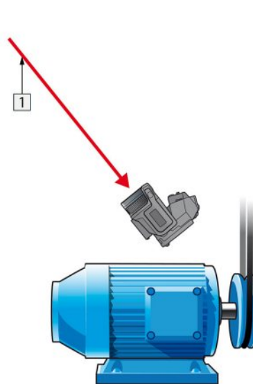
Figure 15.3 1 = Reflection source
