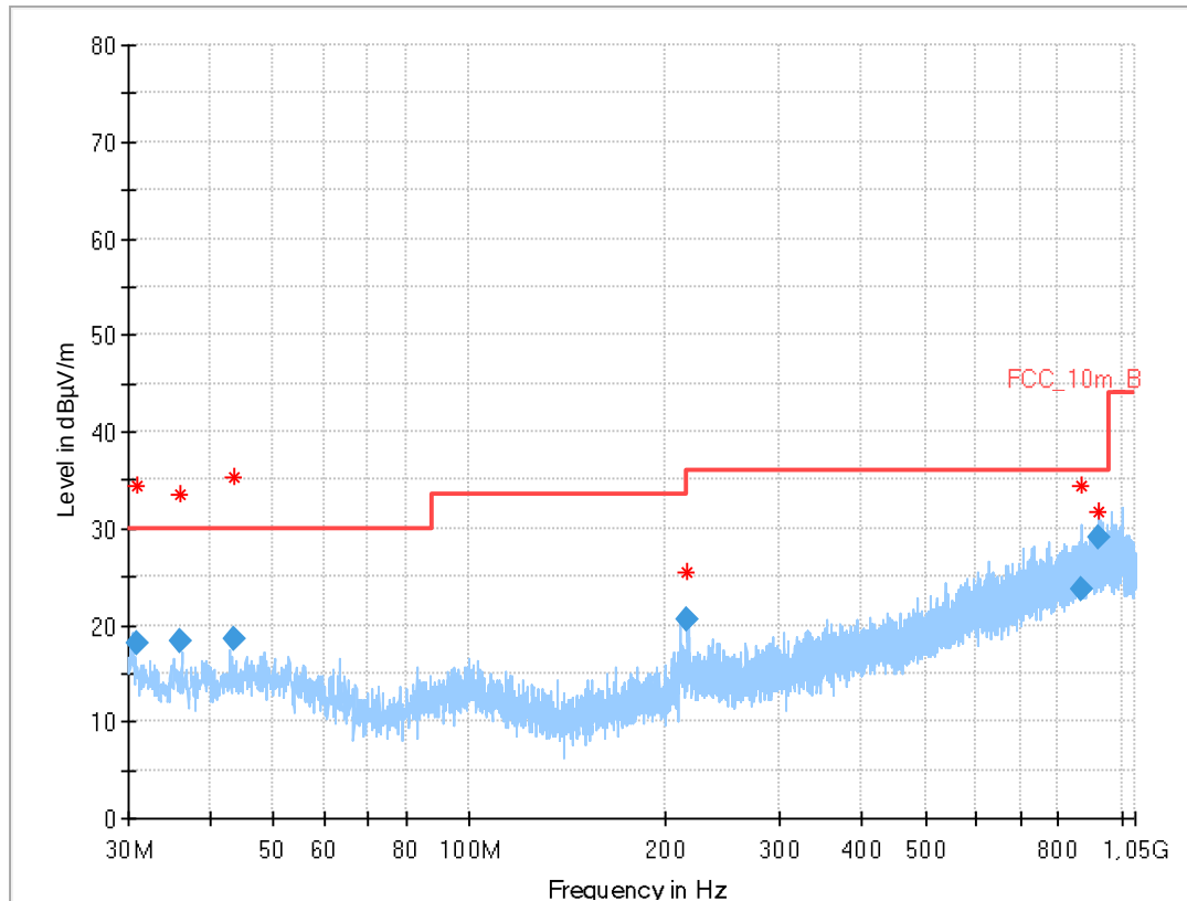
Plot 4: 30 MHz to 1 GHz; vertical & horizontal polarization; cabinet radiation
