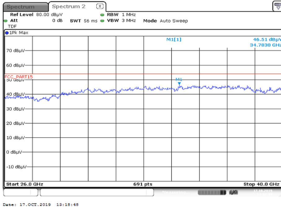
Plot 3: 26 GHz to 40 GHz; vertical & horizontal polarization; U-NII-1 & U-NII-2A; cabinet radiation
