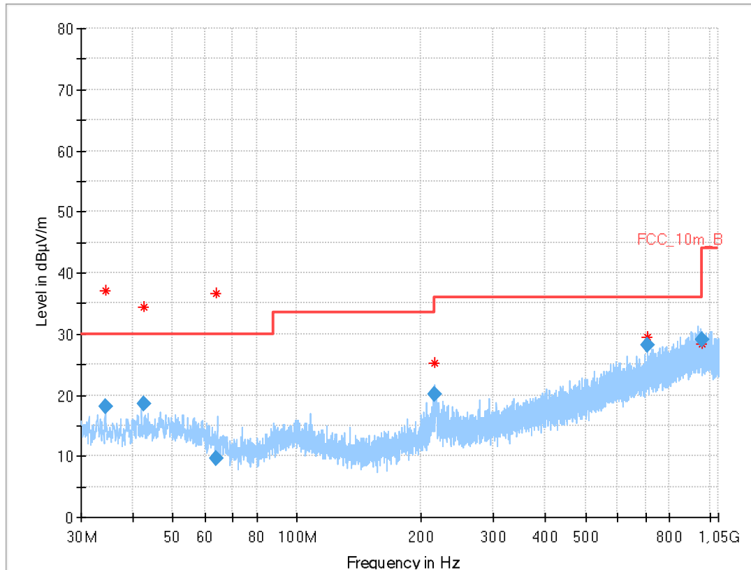
Plot 2: 30 MHz to 1 GHz; vertical & horizontal polarization; U-NII-1; middle channel
