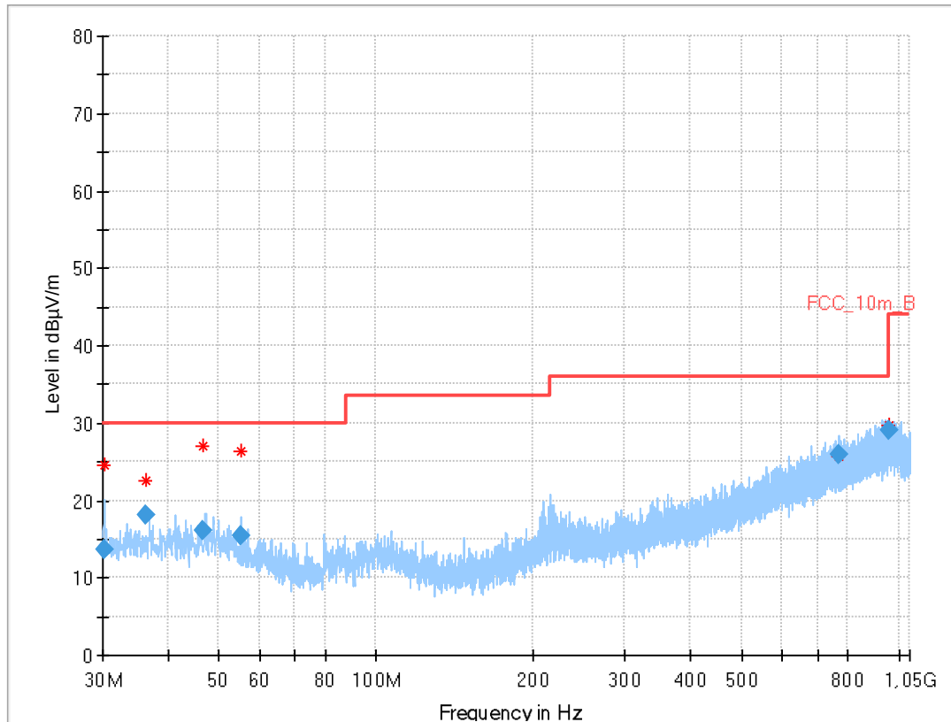
Plot 3: 30 MHz to 1 GHz; vertical & horizontal polarization; U-NII-1; highest channel
