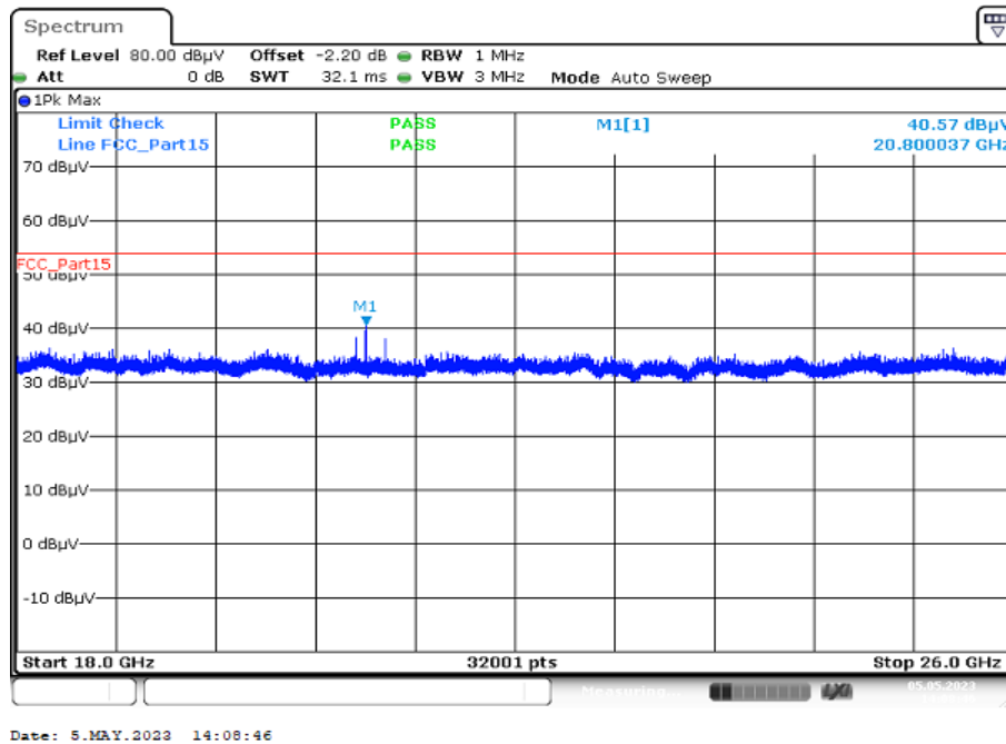
Plot 5: 18 GHz to 26 GHz; vertical &amp; horizontal polarization; U-NII-1; middle channel
