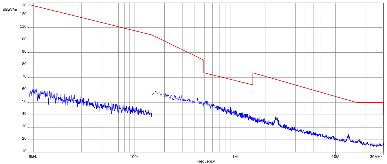
Plot 6: 9 kHz to 30 MHz, U-NII-1; highest channel
