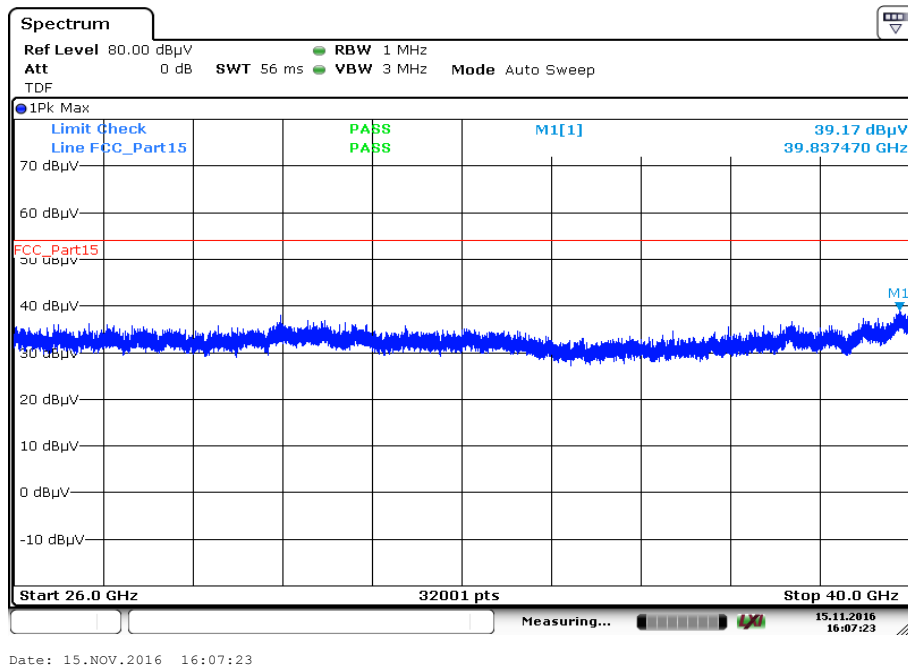
Plot 6: 26 GHz to 40 GHz, vertical & horizontal polarization
