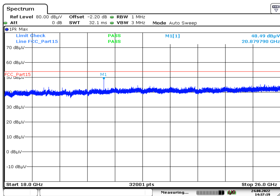
Plot 4: 18 GHz to 26 GHz, TX mode, vertical & horizontal polarization, 1 Msps, valid for all channels
