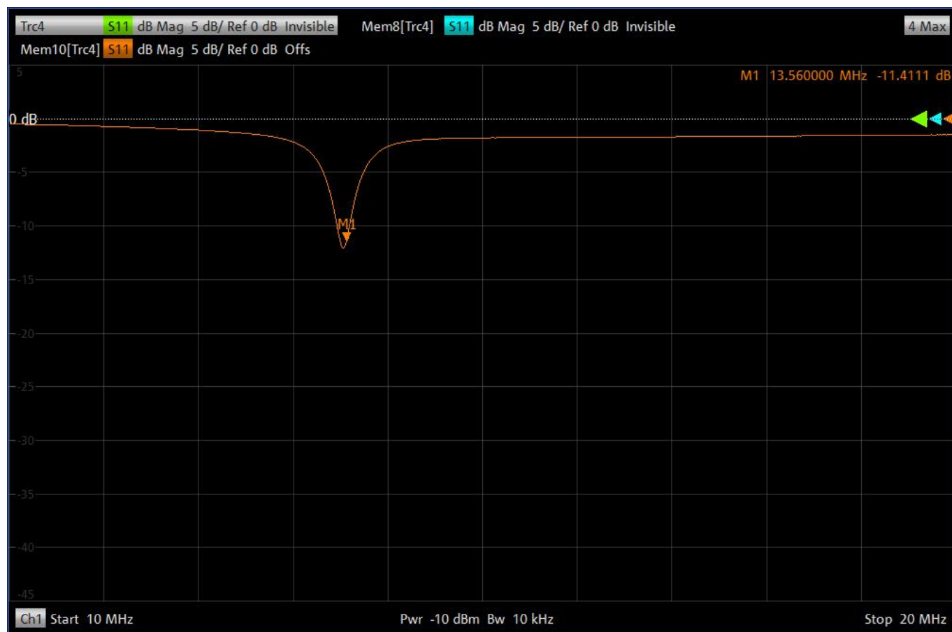
Figure 2 S11
